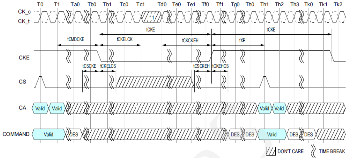
Figure 134 - Basic Power-down Entry and Exit Timing
