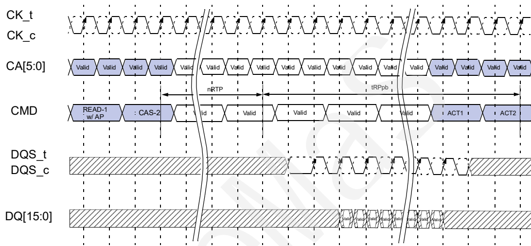
Figure 57 - Burst Read with Auto-Precharge (BL16, Toggling preamble)
