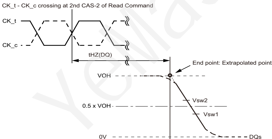
Figure 15 - tHZ(DQ) method for calculating transitions and end point
