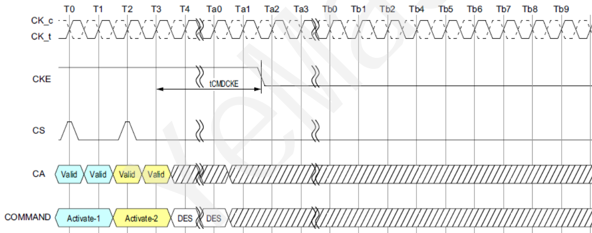
Figure 139 - Activate Command to Power-Down Entry
