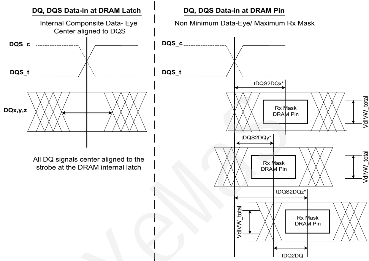
Figure 177 - DQ to DQS (tDQS2DQ and tDQDQ) Timings at the DRAM pins referenced from the internal latch
