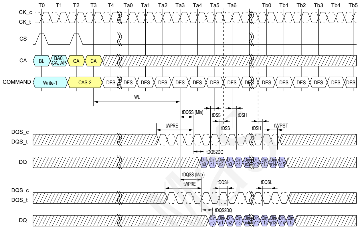
Figure 23 - Write Timing
