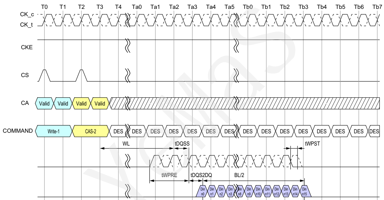
Figure 19 - DQS Write Preamble and Postamble; 0.5nCK Postamble
