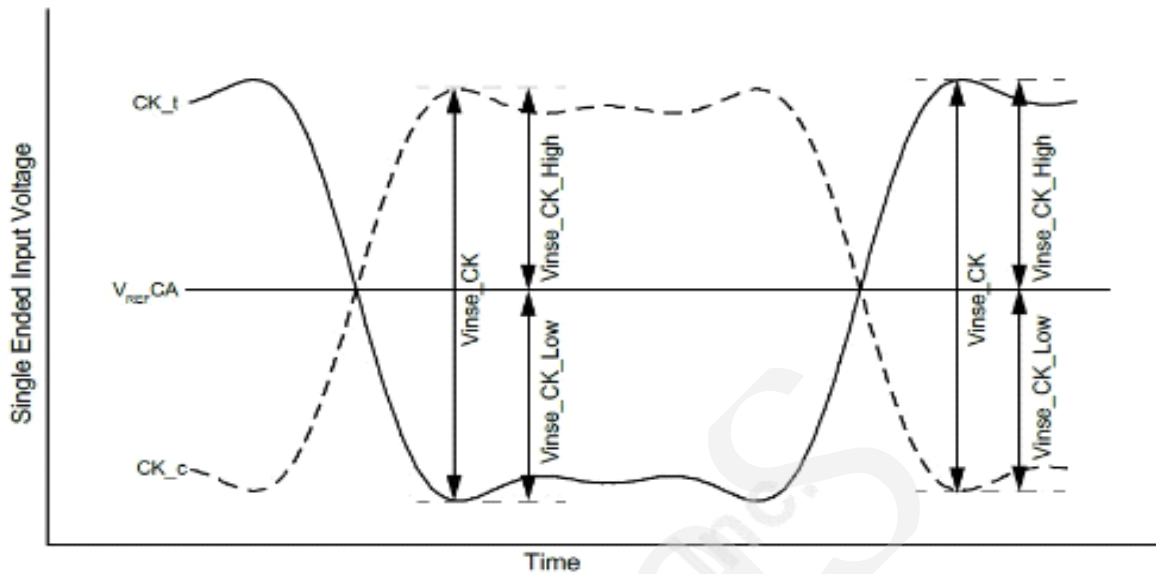
Figure 151 - Clock Single-Ended Input Voltage
