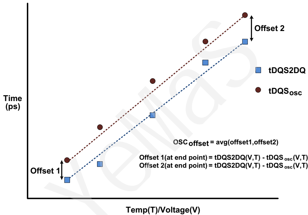
Figure 117 - Interval oscillator offset ( OSC_{offset} )
