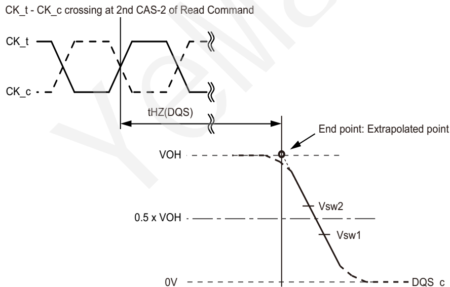
Figure 13 - tHZ(DQS) method for calculating transitions and end point
