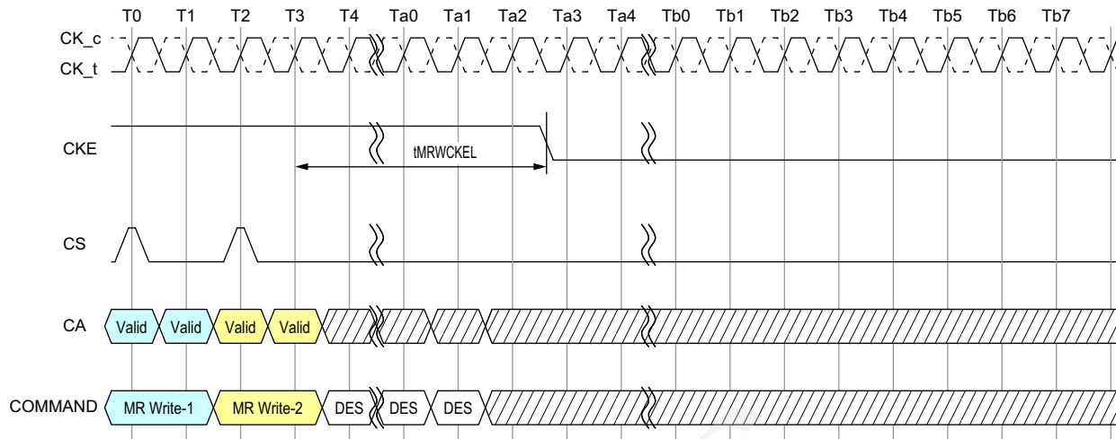
Figure 142 - MRW to Power-Down Entry
