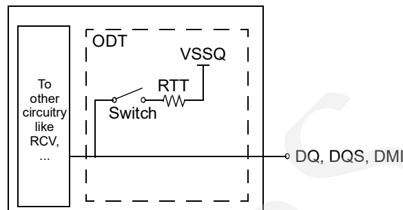
Figure 130 - Functional Representation of ODT
