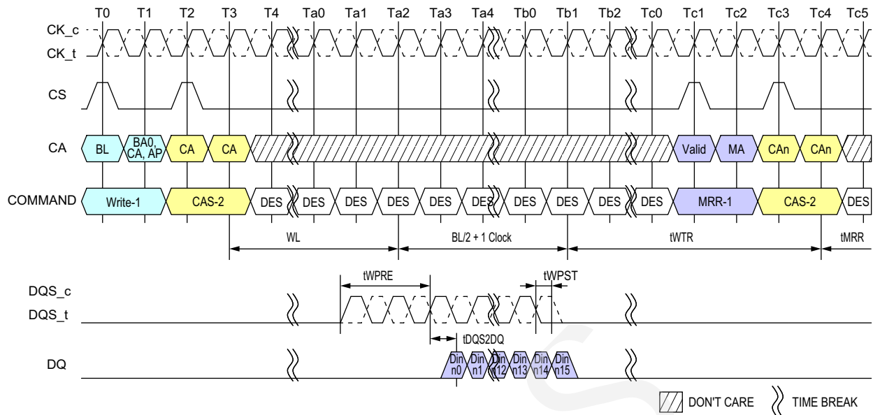
Figure 79 - Write to MRR Timing
