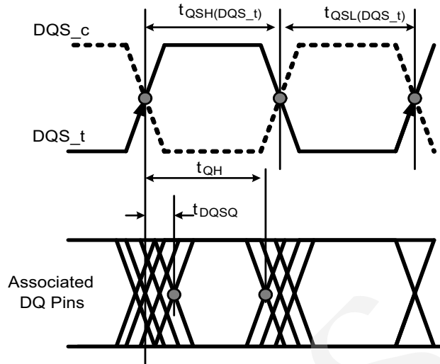
Figure 173 - Read data timing definitions t_{QH} and t_{DQSQ} across on DQ signals per DQS group
