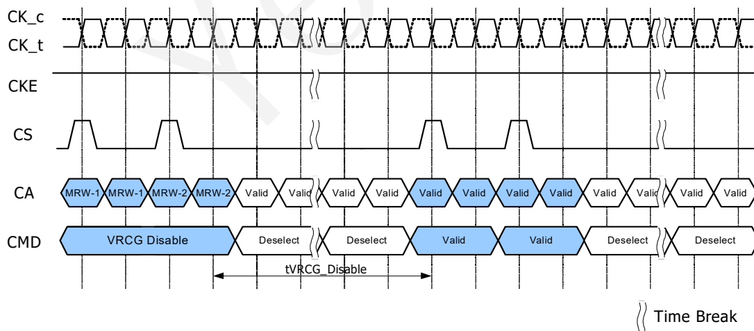
Figure 83 - VRCG Disable timing
