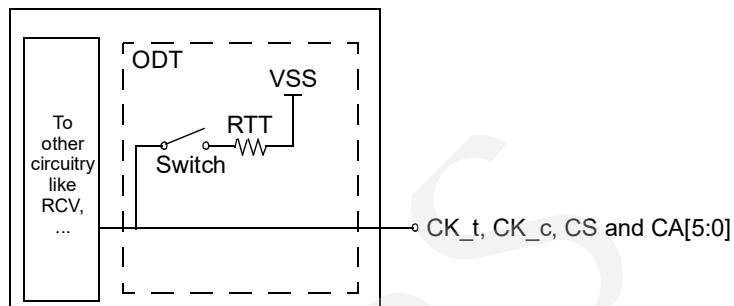
Figure 127 - Functional Representation of CA ODT
