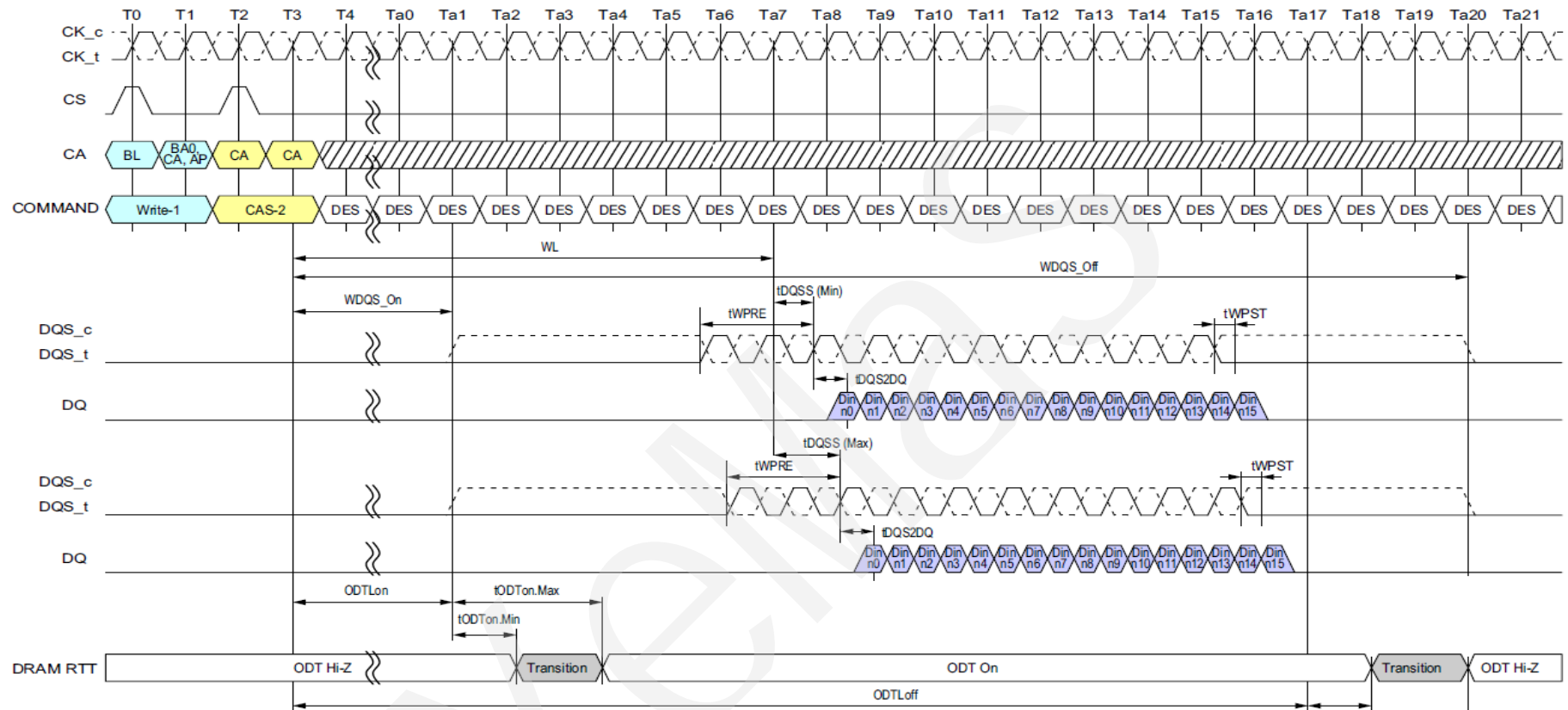
Figure 61 - Burst Write Operation
