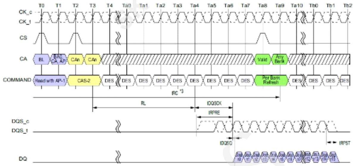
Figure 70 - Burst Read with Auto-Precharge operation followed by Per Bank Refresh
