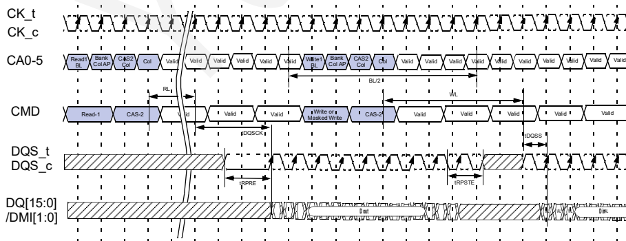
Figure 9 - Burst Read followed by Burst Write. BL=16, Non-toggling tRPRE, Extended tRPST
