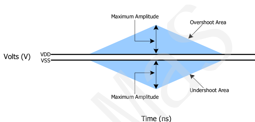
Figure 161 - AC Overshoot and Undershoot Definition
