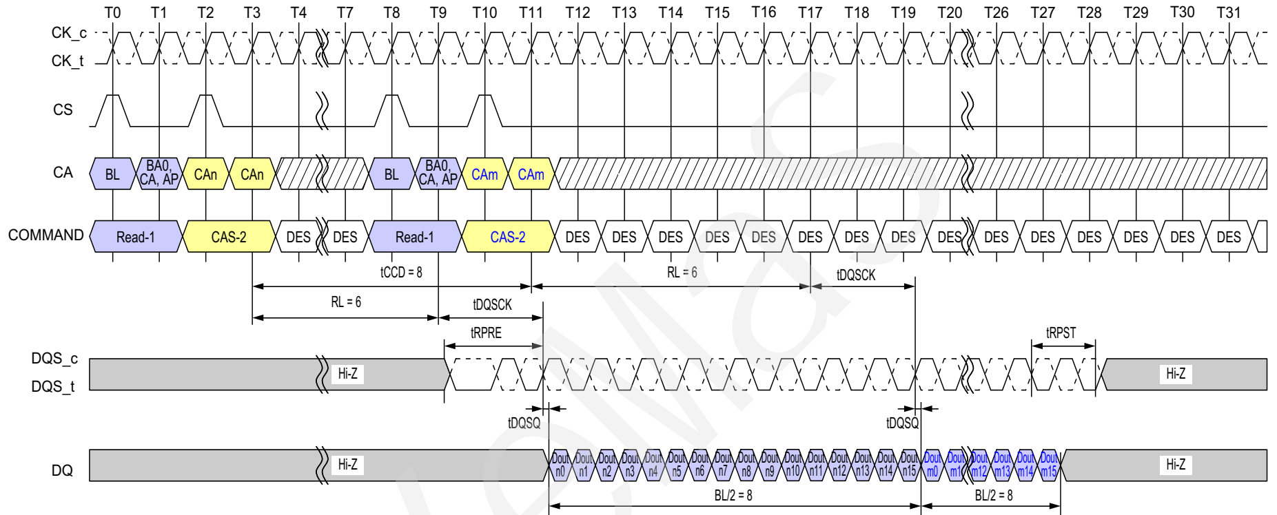
Figure 26 - Seamless Reads Operation: t_{CCD} = \text{Min} , Preamble = Toggle, 1.5nCK Postamble
