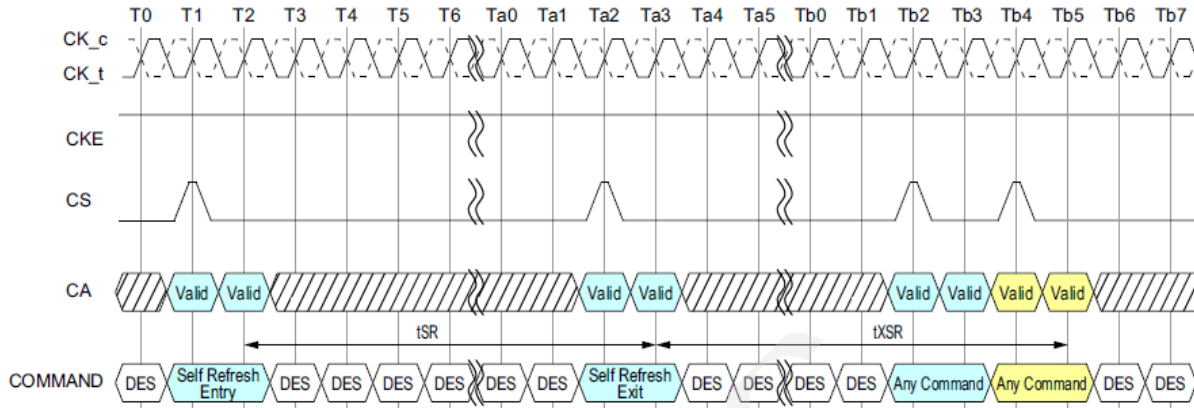
Figure 72 - Self Refresh Entry/Exit Timing
