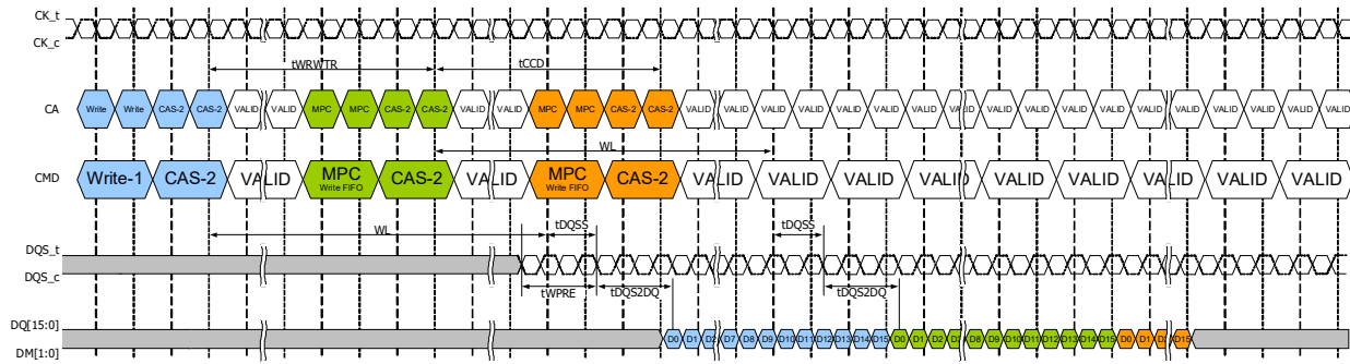
Figure 121 - MPC [WR FIFO] Operation :WPRE = 2nCK, tWPST = 0.5nCK
