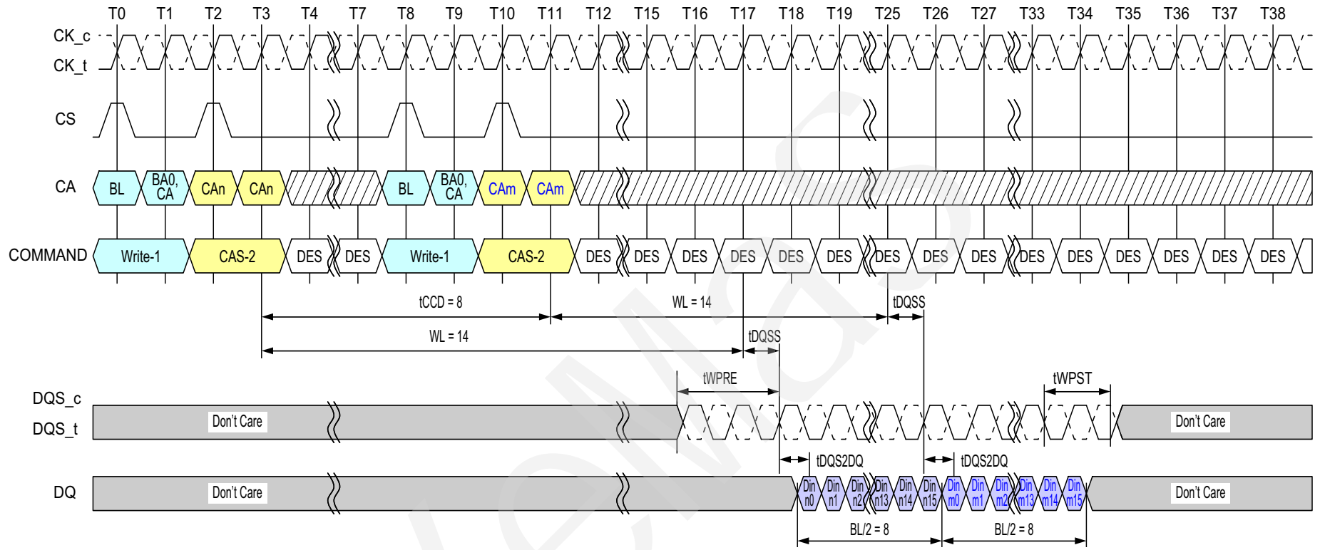
Figure 41 - Seamless Writes Operation: t_{CCD} = \text{Min}, 1.5n\text{CK} Postamble
