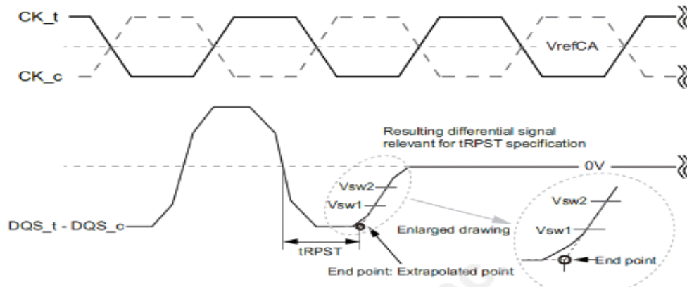
Figure 18 - Method for calculating tRPST transitions and endpoints
