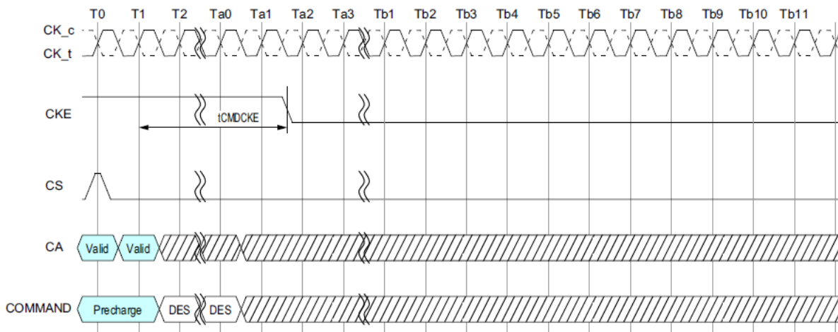
Figure 140 - Precharge Command to Power-Down Entry
