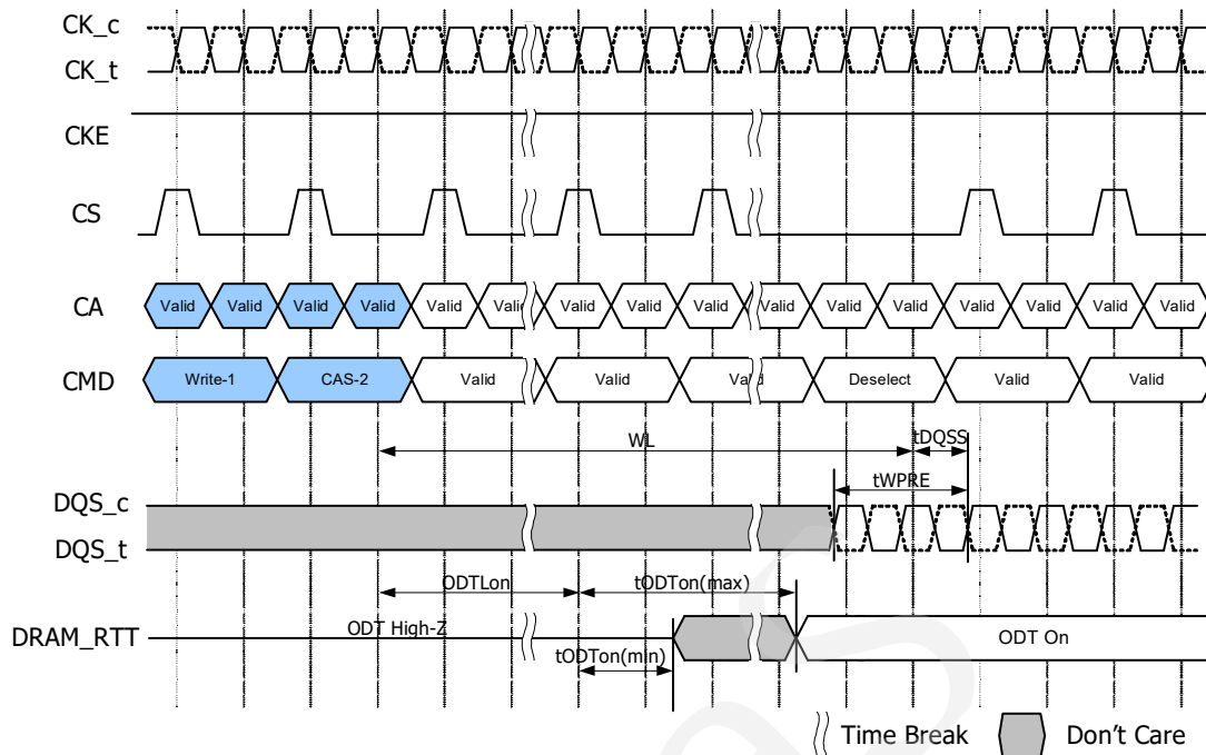
Figure 131 - Asynchronous ODT ON Timing Example; tWPRE = 2 tCK, tDQSS = Nominal
