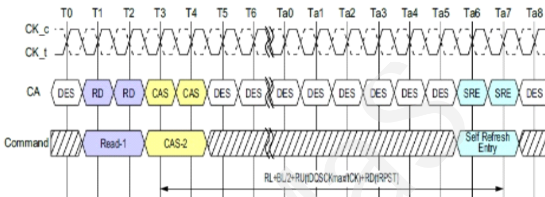
Figure 71 - Self Refresh Entry and Exit
