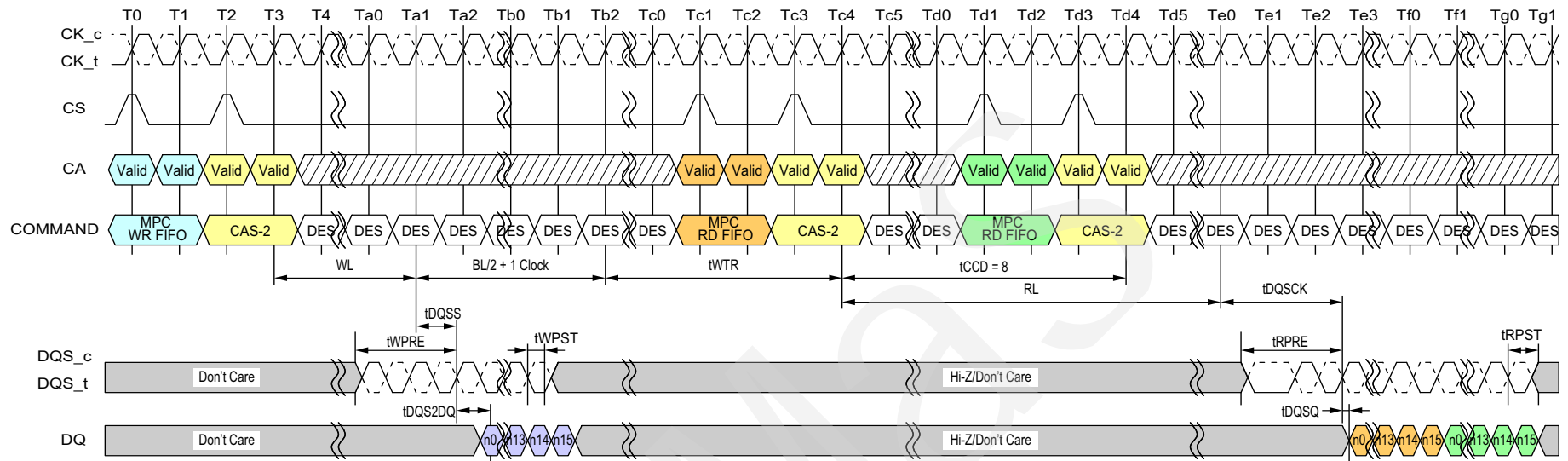
Figure 113 - MPC [Write FIFO] to MPC [Read FIFO] Timing
