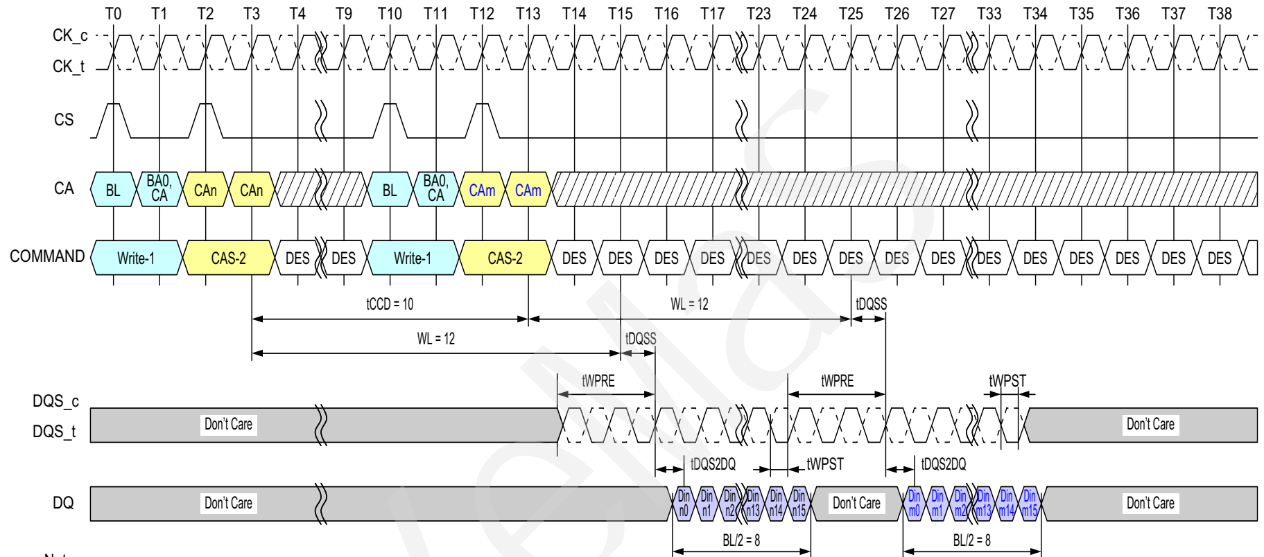
Figure 44 - Consecutive Writes Operation: t_{CCD} = \text{Min} + 2, 0.5n\text{CK} Postamble
