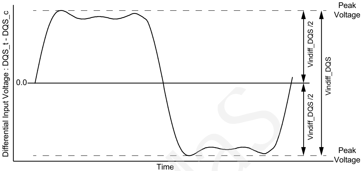
Figure 154 - DQS Differential Input Voltage
