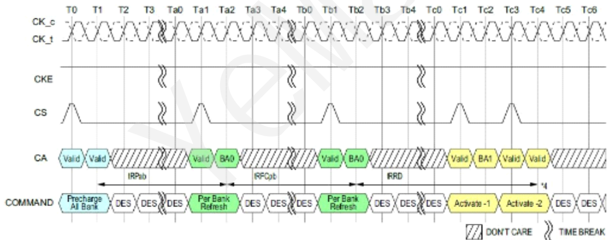
Figure 66 - Per-Bank REFRESH to a same bank Operation
