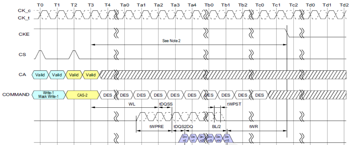
Figure 136 - Write and Mask Write to Power-Down Entry
