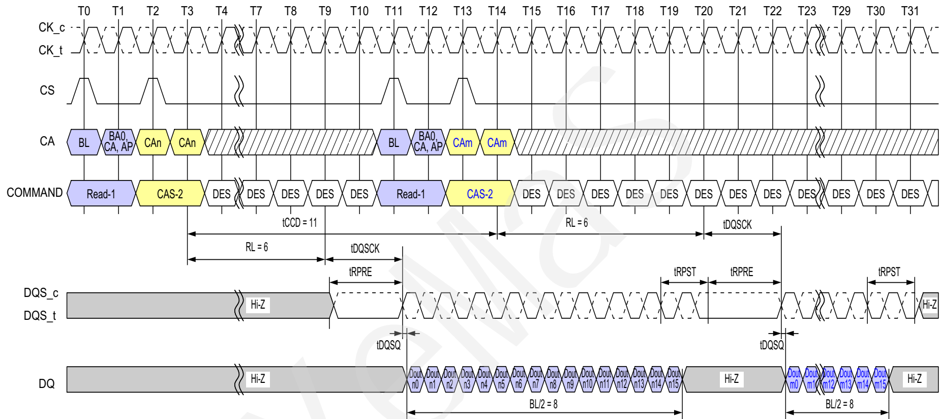
Figure 37 - Consecutive Reads Operation: t_{CCD} = \text{Min} + 3 , Preamble = Static, 1.5nCK Postamble
