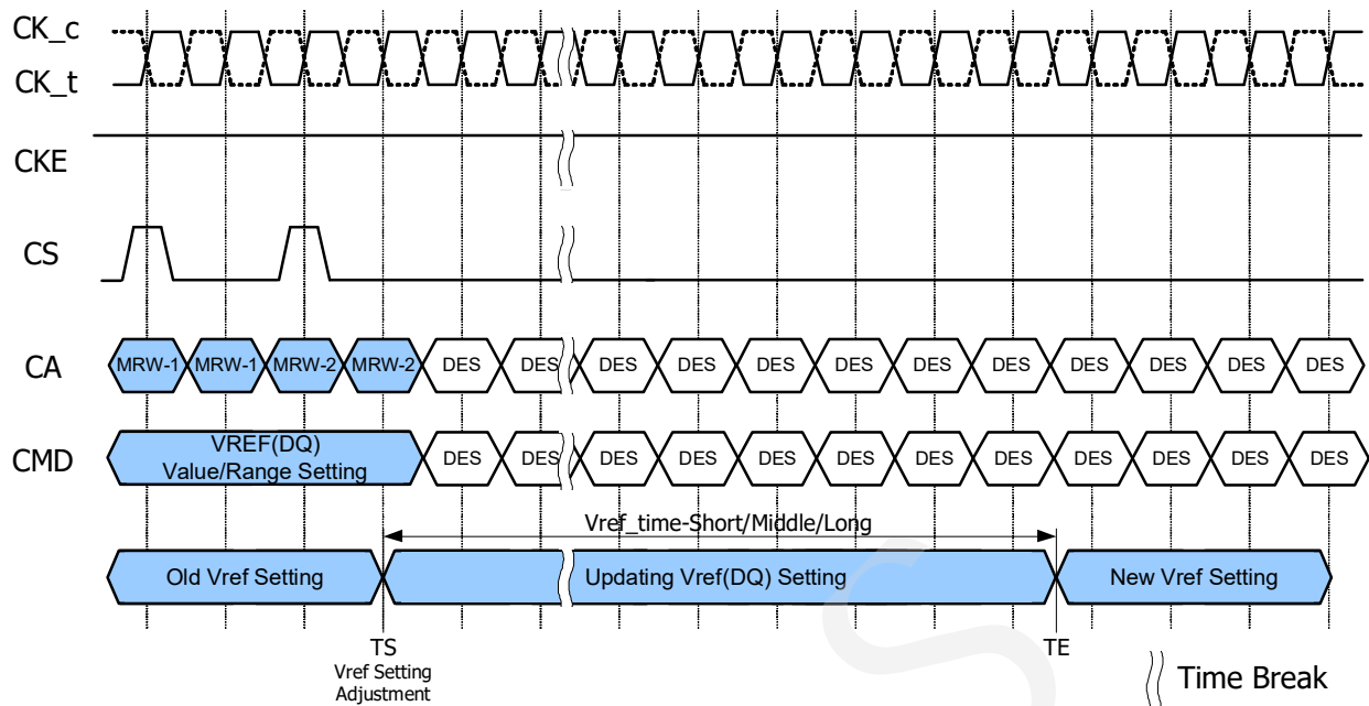
Figure 93 - Vref_time for short and long timing diagram
