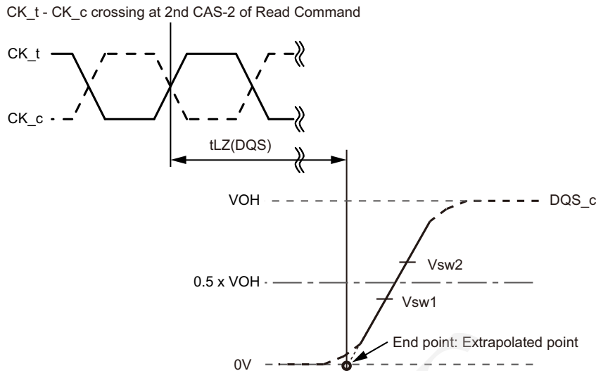
Figure 12 - tLZ(DQS) method for calculating transitions and end point
