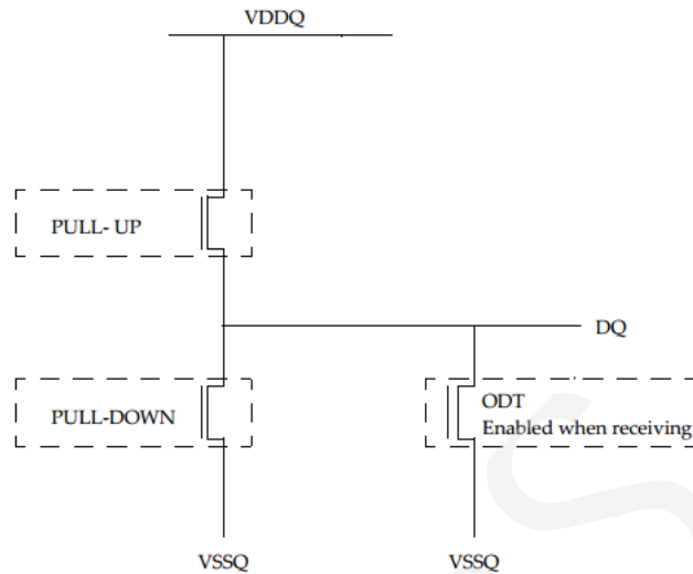
Figure 163 - LVSTL I/O Cell
