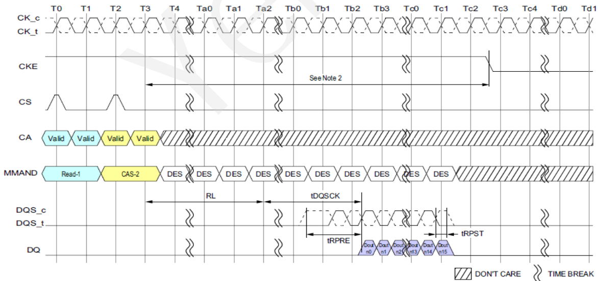
Figure 135 - Read and Read with Auto-precharge to Power-Down Entry
