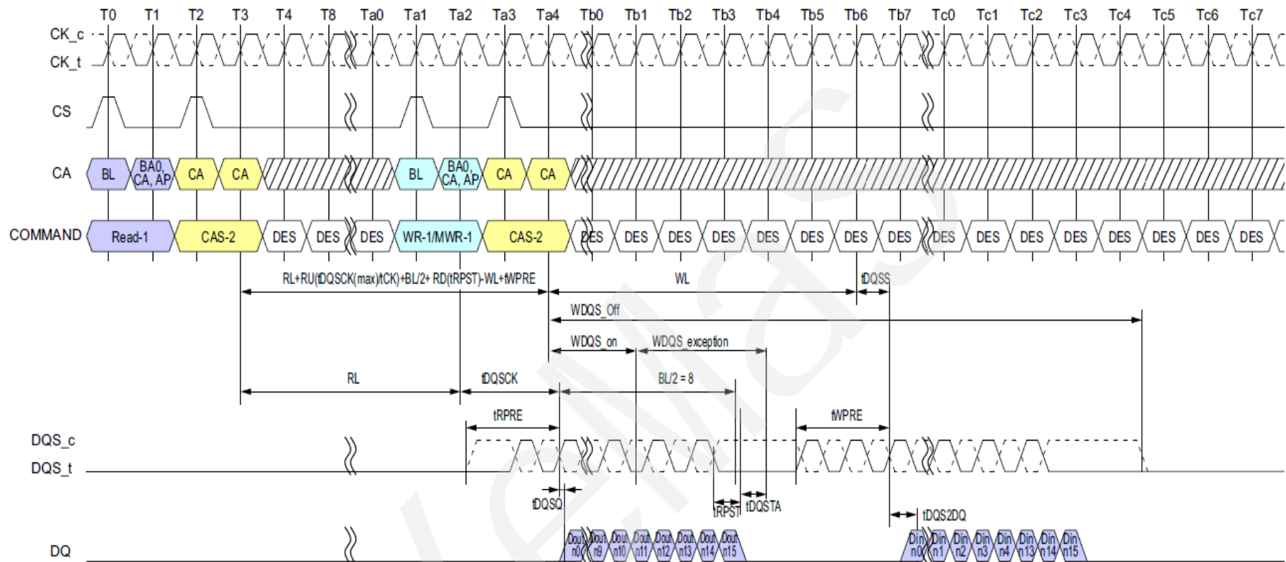
Figure 62 - Burst Read followed by Burst Write or Burst Mask Write (ODT Disable)
