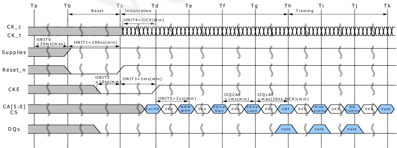
Figure 3 - Power Ramp and Initialization Sequence
