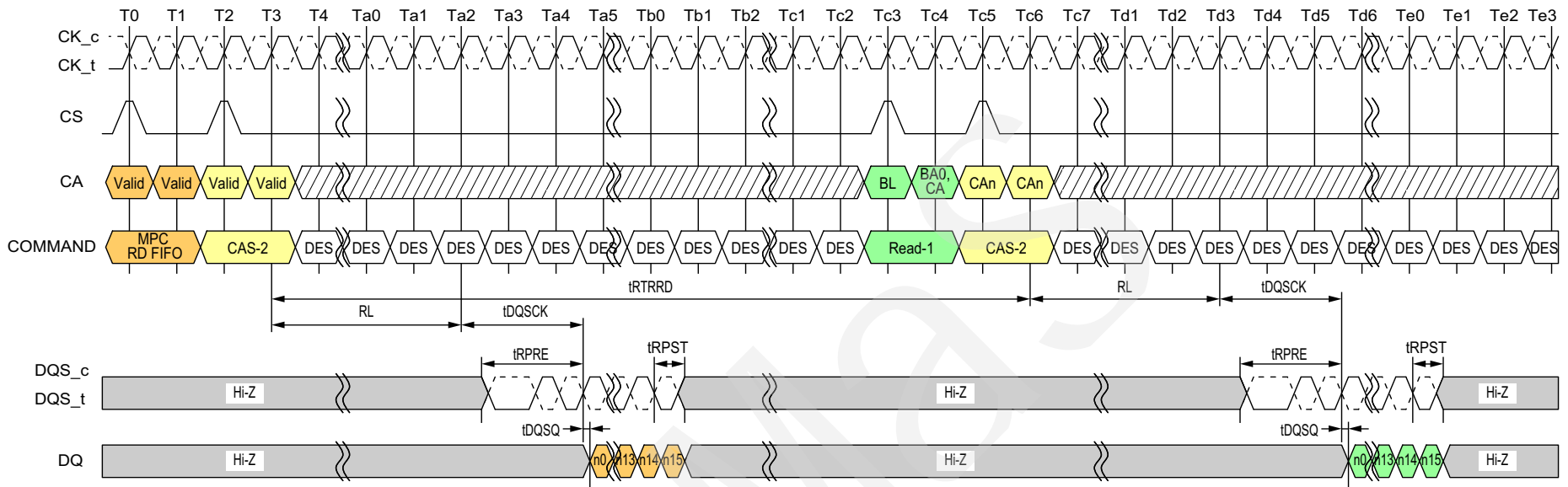
Figure 114 - MPC [Read FIFO] to Read Timing
