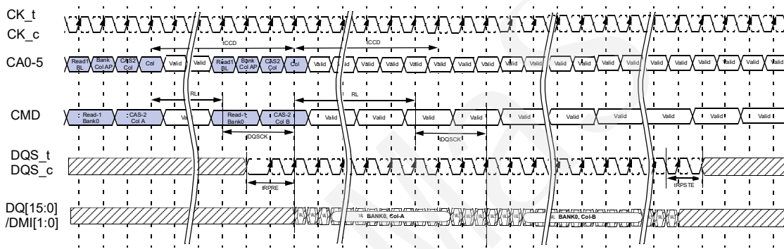
Figure 8 - Burst Read Timing. BL=16, Toggling tRPRE, Extended tRPST
