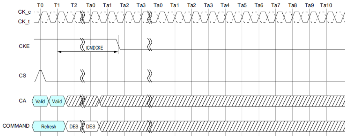
Figure 138 - Refresh entry to Power-Down Entry
