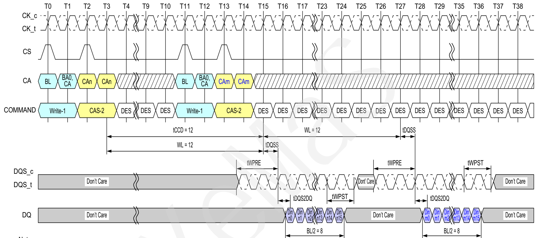
Figure 48 - Consecutive Writes Operation: t_{CCD} = \text{Min} + 4, 1.5n\text{CK} Postamble
