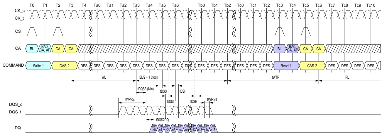
Figure 22 - Burst Write Followed by Burst Read
