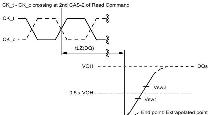
Figure 14 - tLZ(DQ) method for calculating transitions and end point
