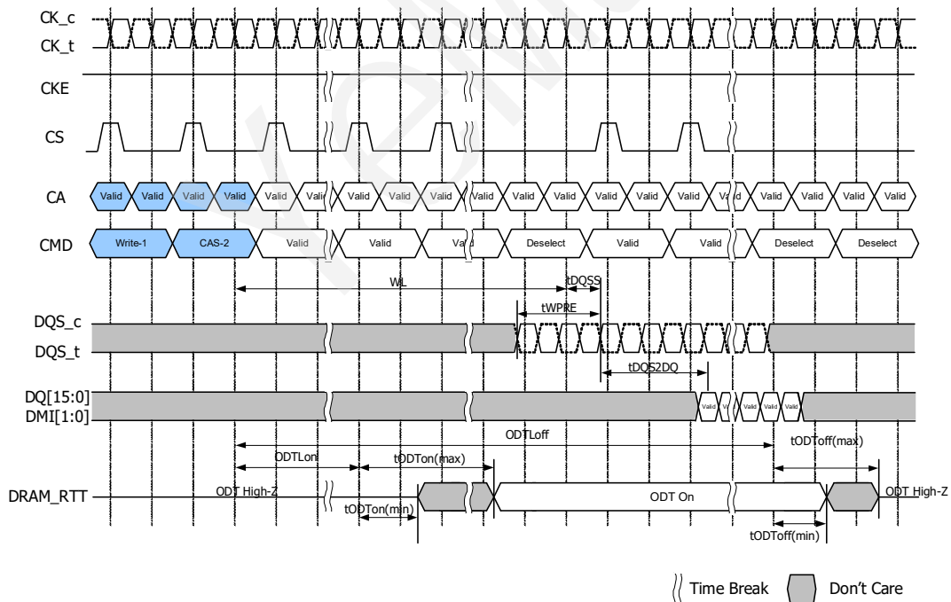
Figure 132 - Asynchronous ODT OFF Timing Example, tWPRE = 2 nCK, tDQSS = Nominal
