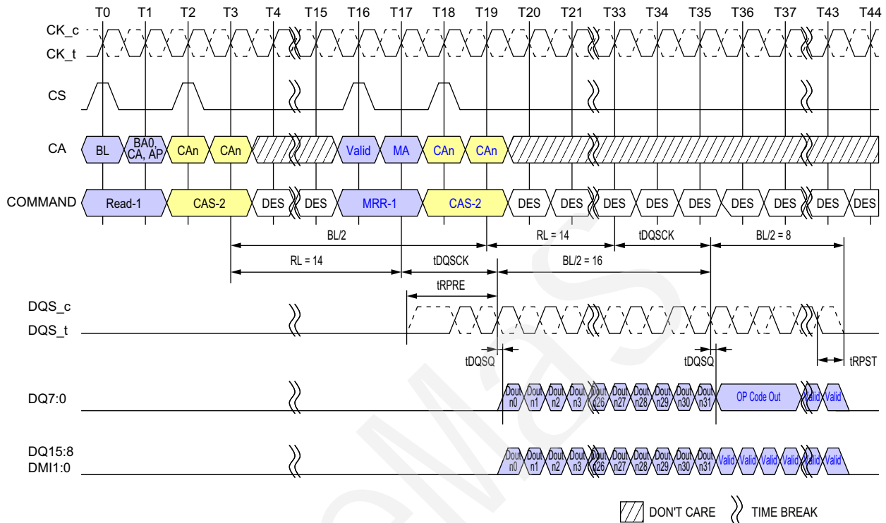
Figure 78 - Read to MRR Timing
