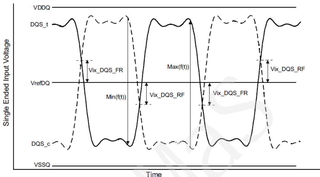
Figure 158 - Vix Definition (DQS)
