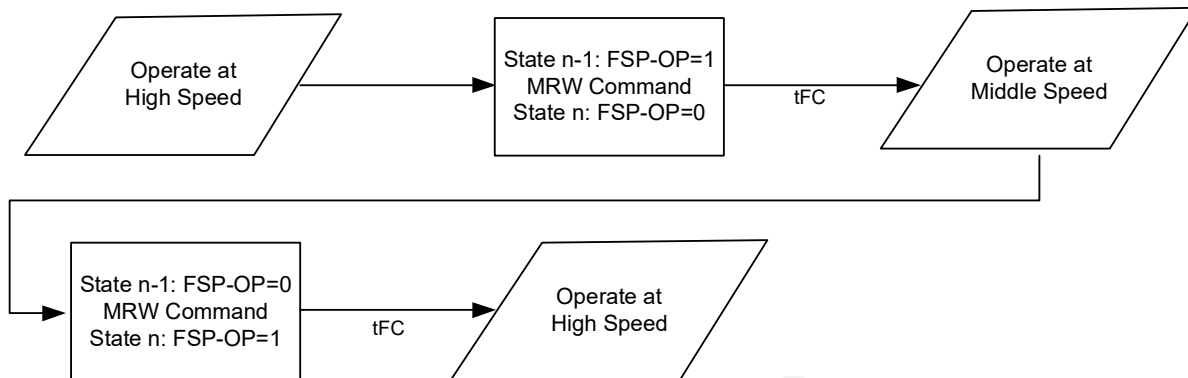
Figure 104 - Switching between two trained Frequency Set Points
