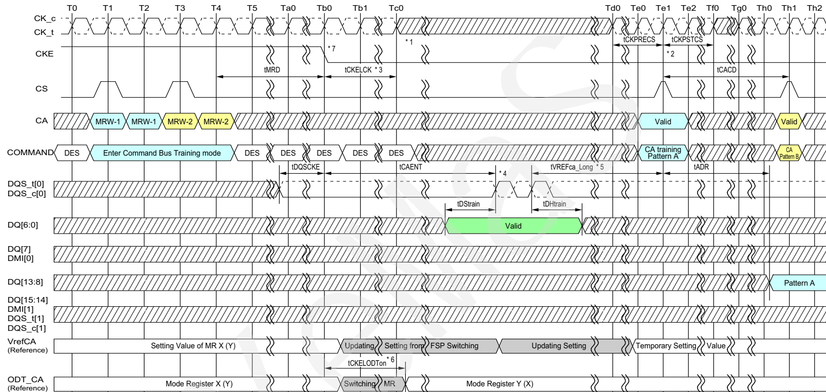
Figure 98 - Entering Command Bus Training Mode and CA Training Pattern Input and Output
