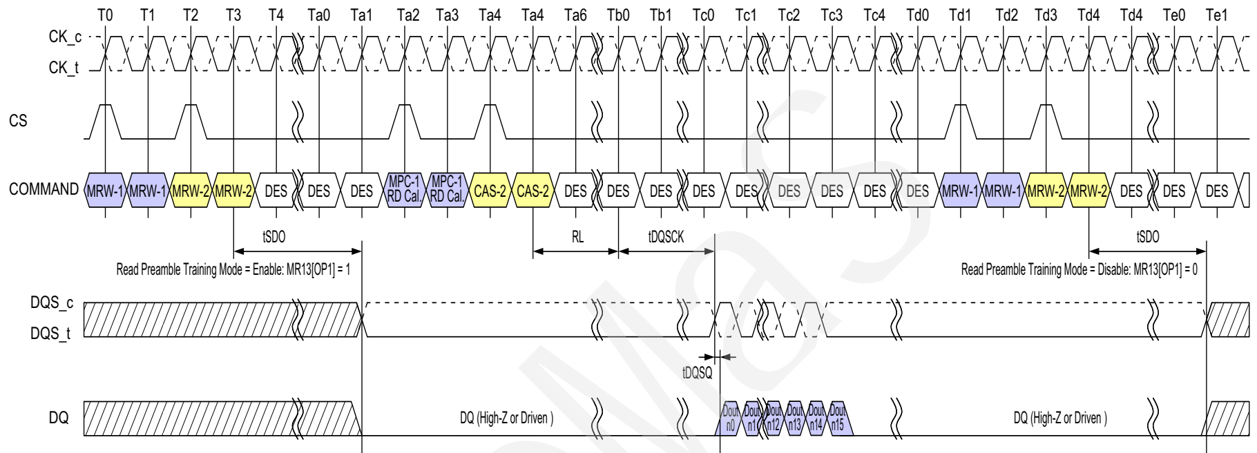
Figure 120 - Read Preamble Training
