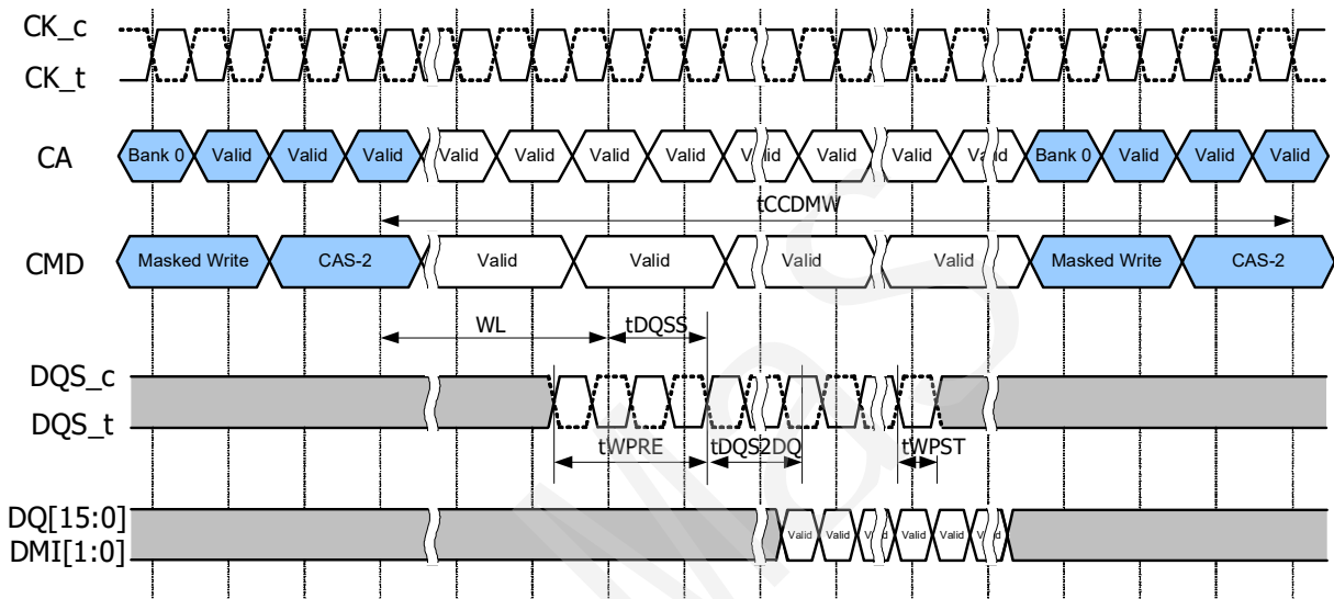
Figure 49 - Masked Write Command - Same Bank (Shown with BL16, 2tCK Preamble)
