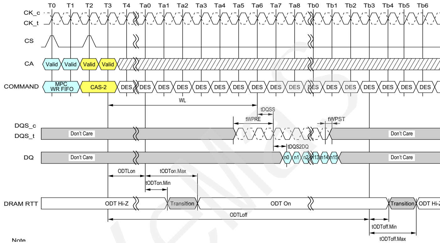
Figure 115 - MPC [Write FIFO] with DQ ODT Timing
