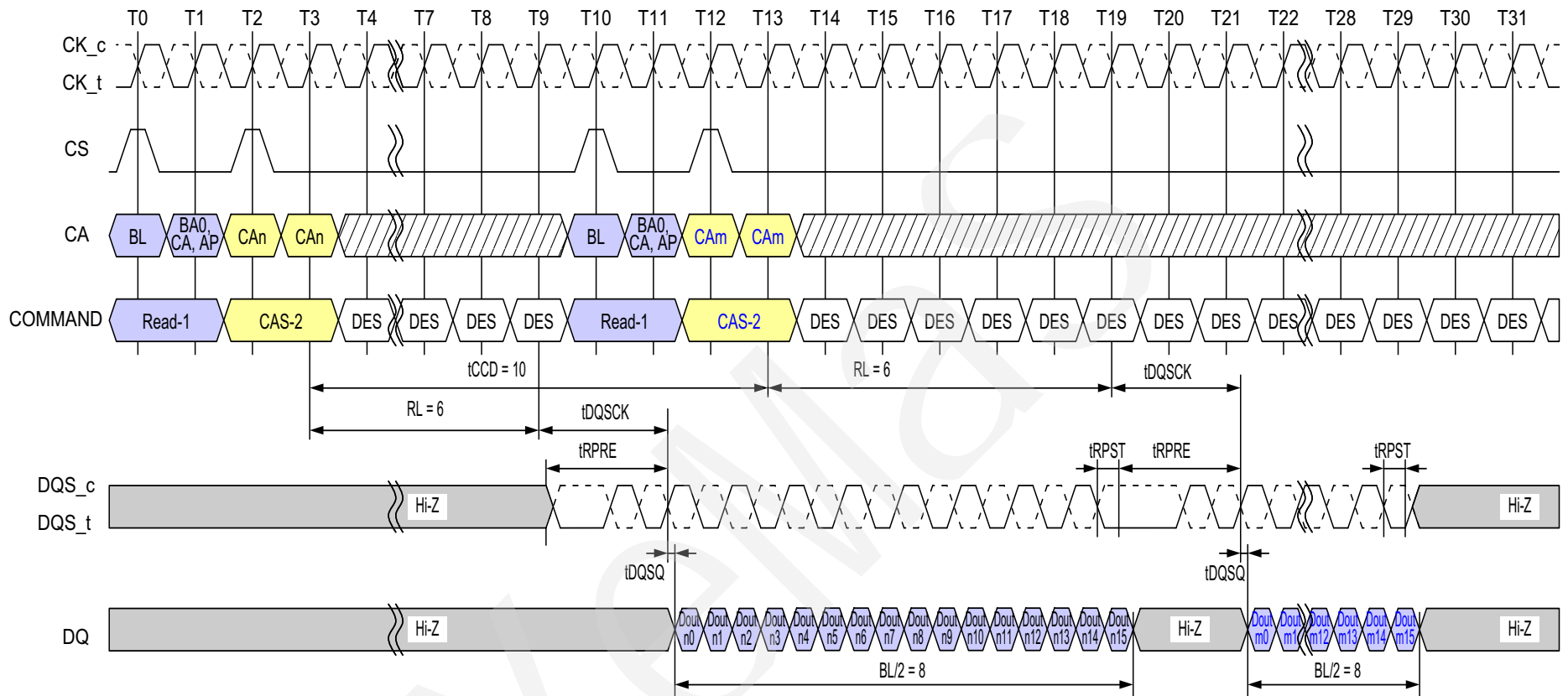
Figure 32 - Consecutive Reads Operation: t_{CCD} = \text{Min} + 2 , Preamble = Toggle, 0.5n\text{CK} Postamble
