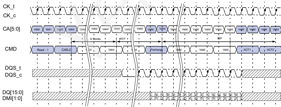
Figure 54 - Burst Read followed by Precharge (BL32, Toggling Preamble)
