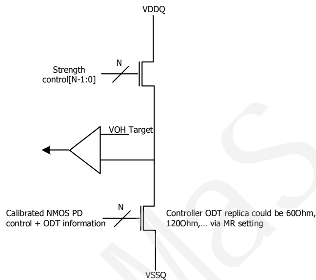
Figure 165 - Pull-up calibration
