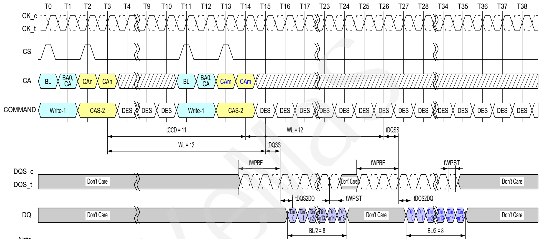
Figure 46 - Consecutive Writes Operation: t_{CCD} = \text{Min} + 3, 0.5n\text{CK} Postamble
