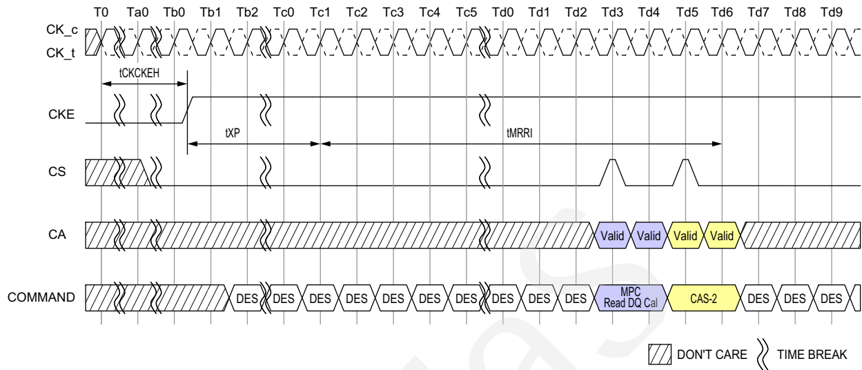
Figure 111 - MPC Read DQ Calibration Following Power-Down State
