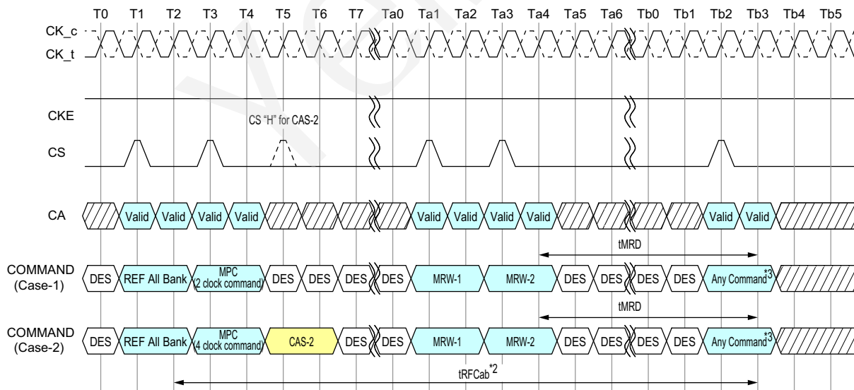
Figure 76 - MRR, MRW and MPC Commands Issuing Timing during tRFC
