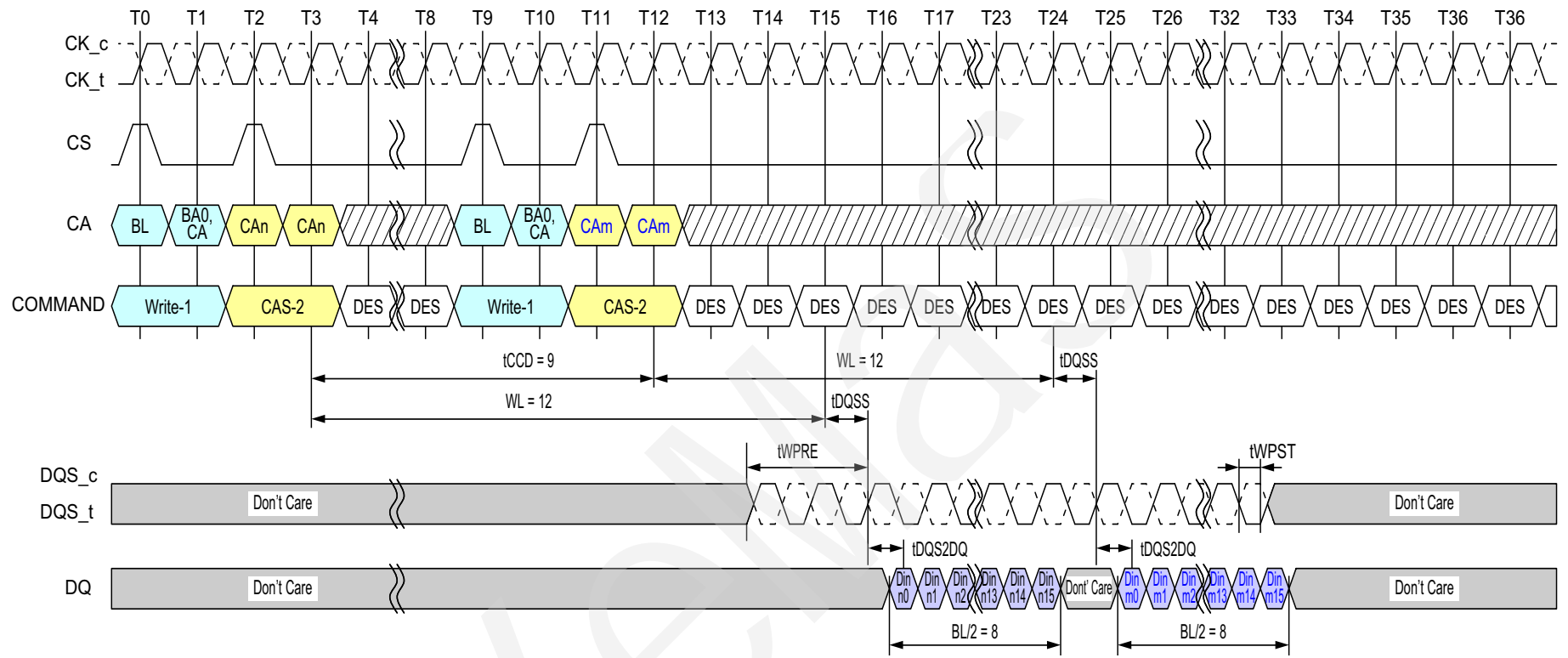
Figure 42 - Consecutive Writes Operation: t_{CCD} = \text{Min} + 1, 0.5n\text{CK} Postamble
