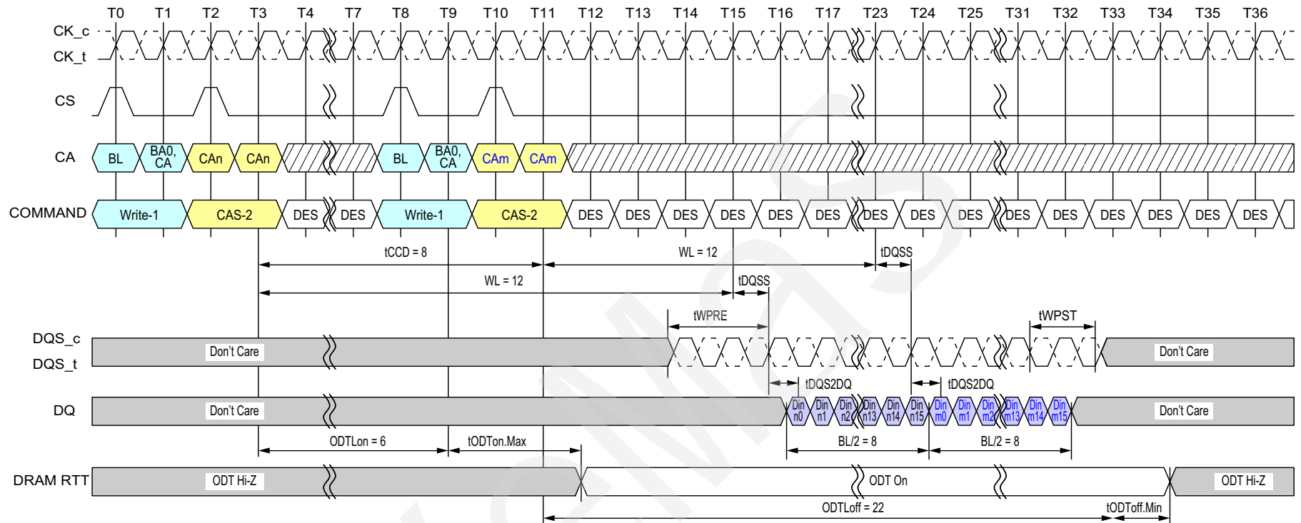
Figure 40 - Seamless Writes Operation: t CCD = Min, 1.5nCK Postamble, 533MHz < Clock Freq. ≤ 800MHz, ODT Worst Timing Case
