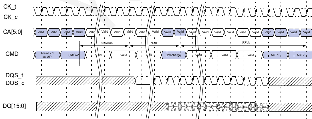
Figure 58 - Burst Read with Auto-Precharge (BL32, Toggling preamble)
