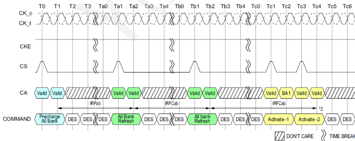
Figure 64 - All-Bank REFRESH Operation
