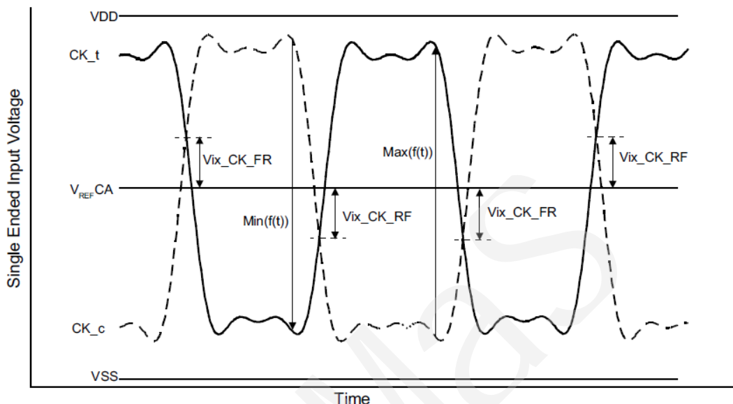
Figure 153 - Vix Definition (Clock)
