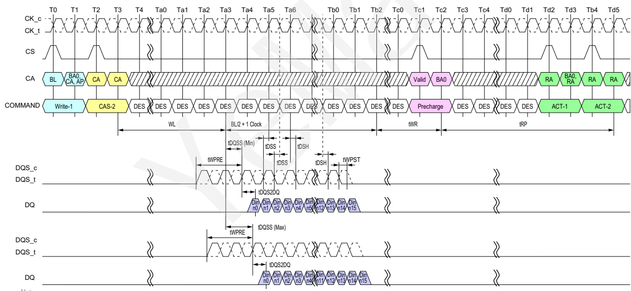
Figure 21 - Burst Write Operation
