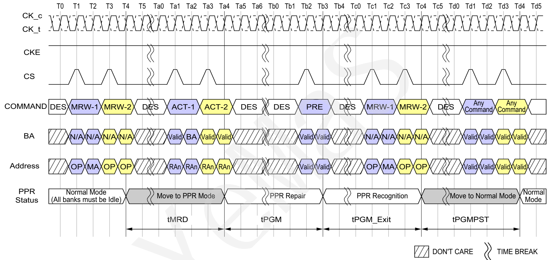
Figure 145 - PPR Timing
