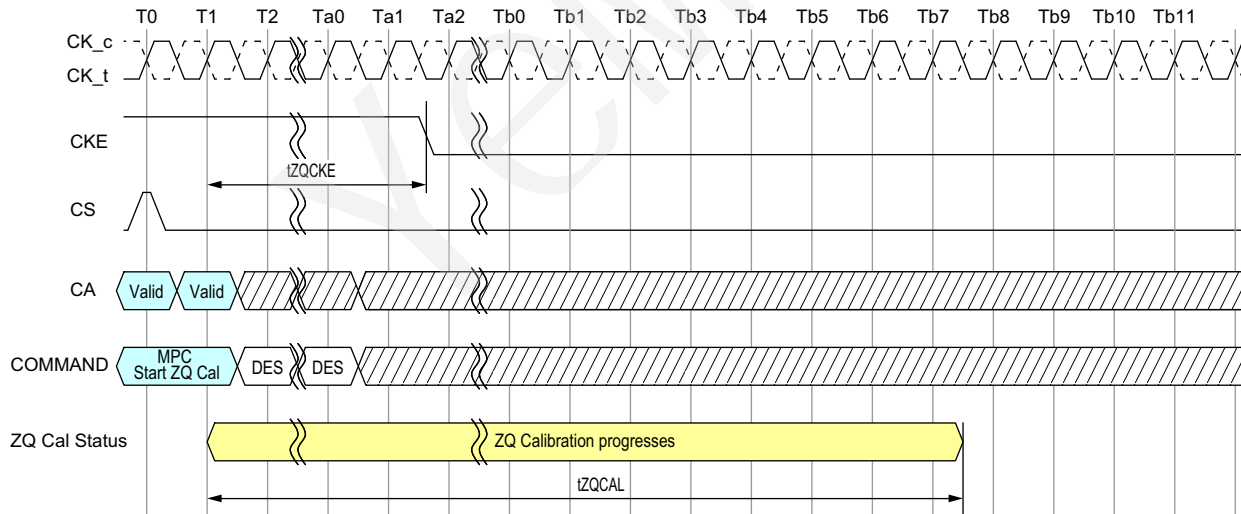
Figure 143 - MPC ZQCAL_start to Power-Down Entry
