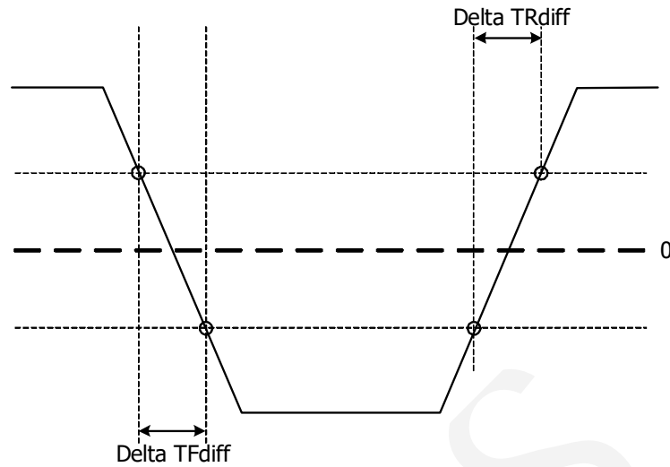
Figure 160 - Differential Output Slew Rate Definition
