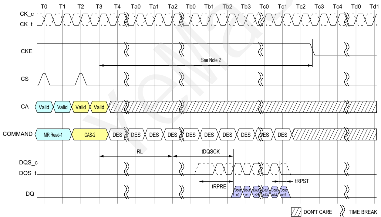
Figure 141 - Mode Register Read to Power-Down Entry
