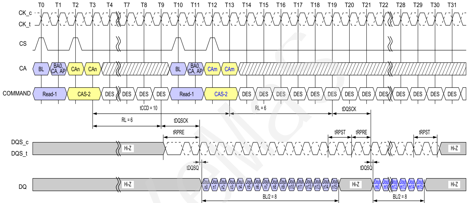
Figure 31 - Consecutive Reads Operation: t_{CCD} = \text{Min} + 2 , Preamble = Toggle, 1.5nCK Postamble
