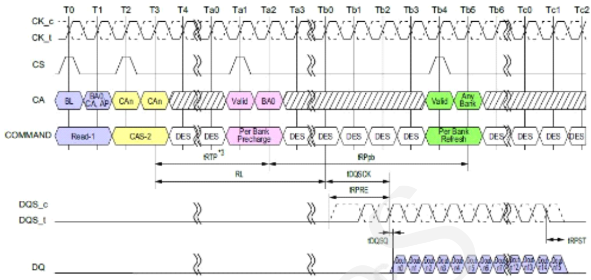
Figure 69 - Burst Read Operation followed by Per Bank Refresh
