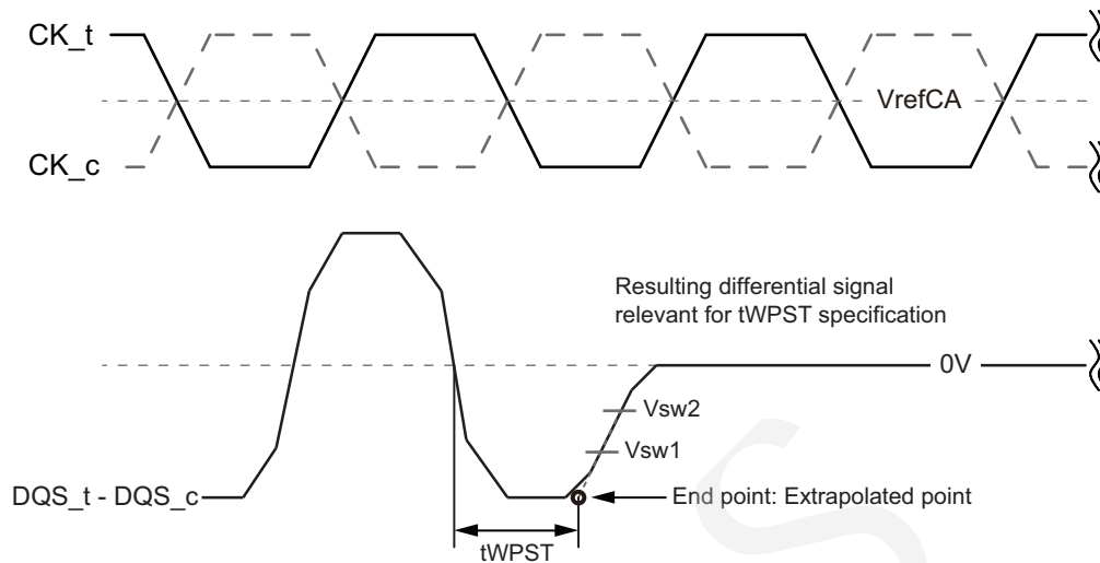
Figure 25 - Method for calculating tWPST transitions and endpoints
