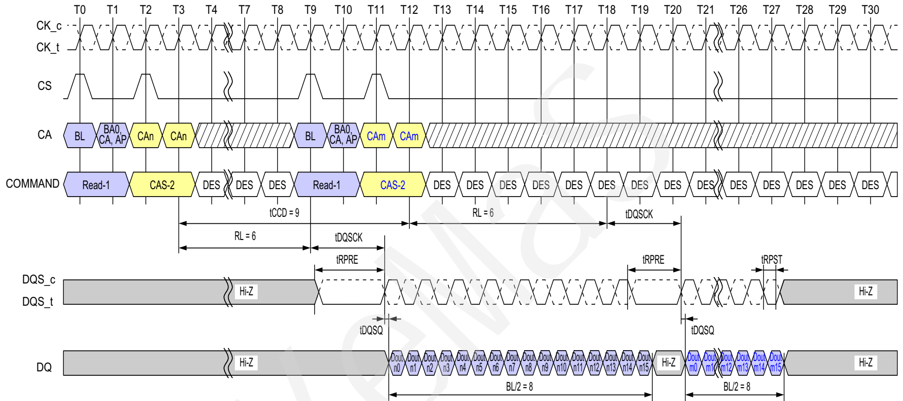
Figure 30 - Consecutive Reads Operation: t_{CCD} = \text{Min} + 1 , Preamble = Static, 0.5n\text{CK} Postamble
