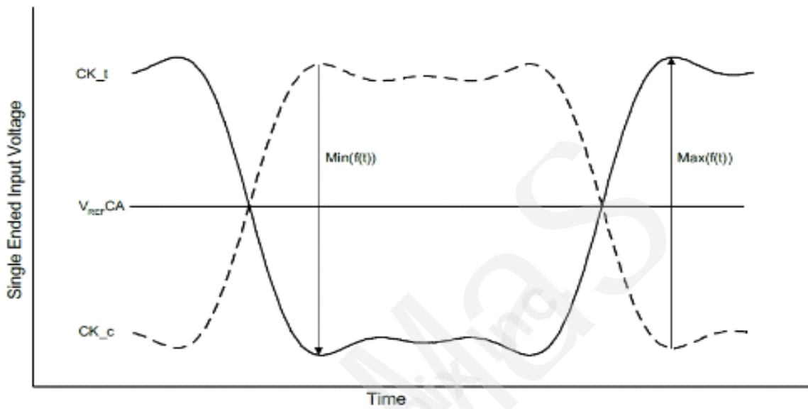
Figure 150 - Definition of differential Clock Peak Voltage
