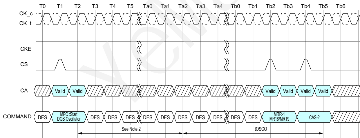
Figure 119 - In case of DQS Interval Oscillator is stopped by DQS interval timer
