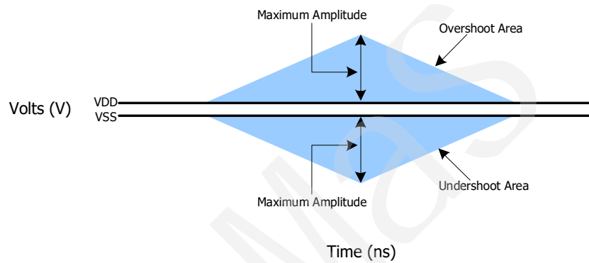
Figure 148 - AC Overshoot and Undershoot Definition for Address and Control Pins
