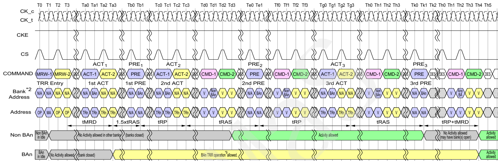
Figure 144 - TRR Mode Timing Example
