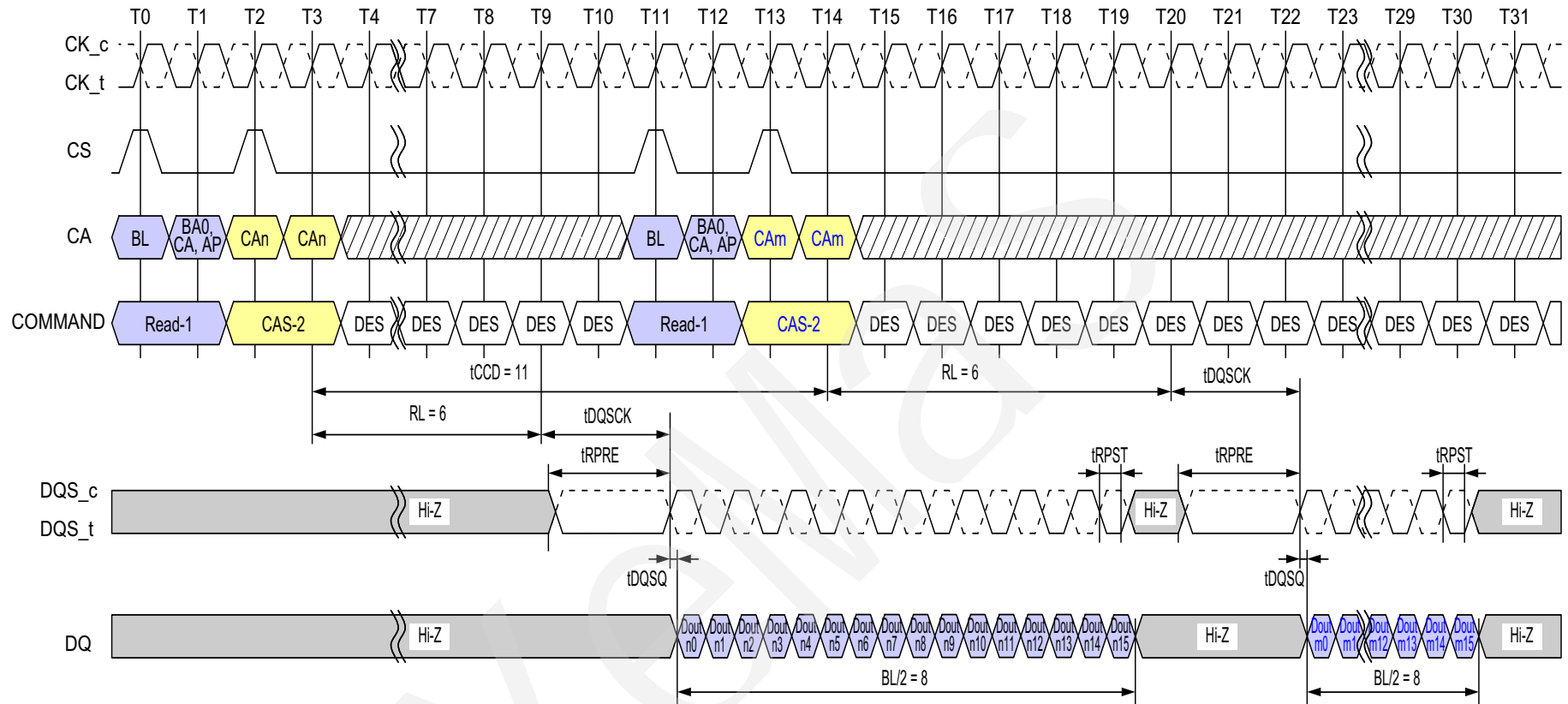
Figure 38 - Consecutive Reads Operation: tCCD = Min +3, Preamble = Static, 0.5nCK Postamble
