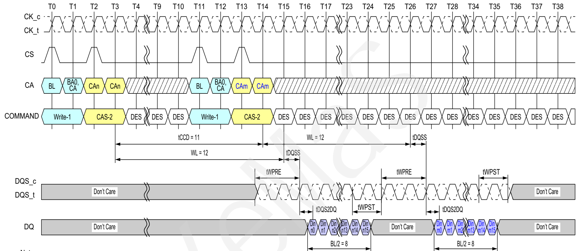
Figure 47 - Consecutive Writes Operation: t_{CCD} = \text{Min} + 3 , 1.5n\text{CK} Postamble
