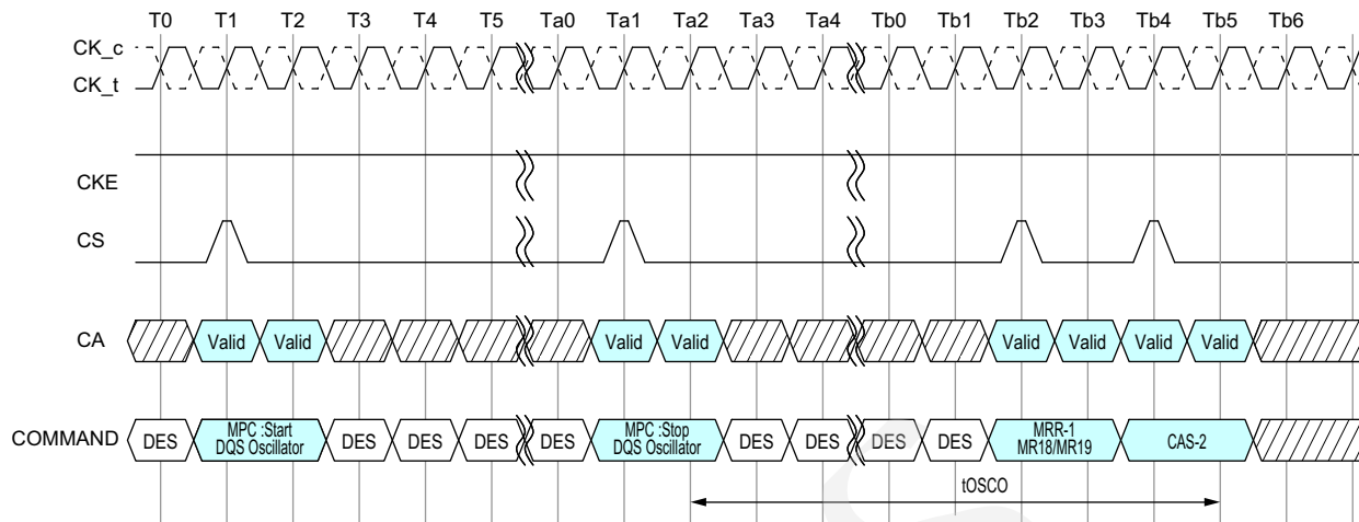
Figure 118 - In case of DQS Interval Oscillator is stopped by MPC Command
