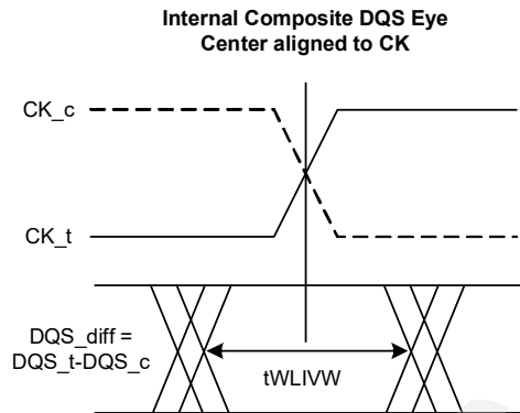
Figure 166 - DQS_t/DQS_c and CK_t/CK_c at DRAM Latch
