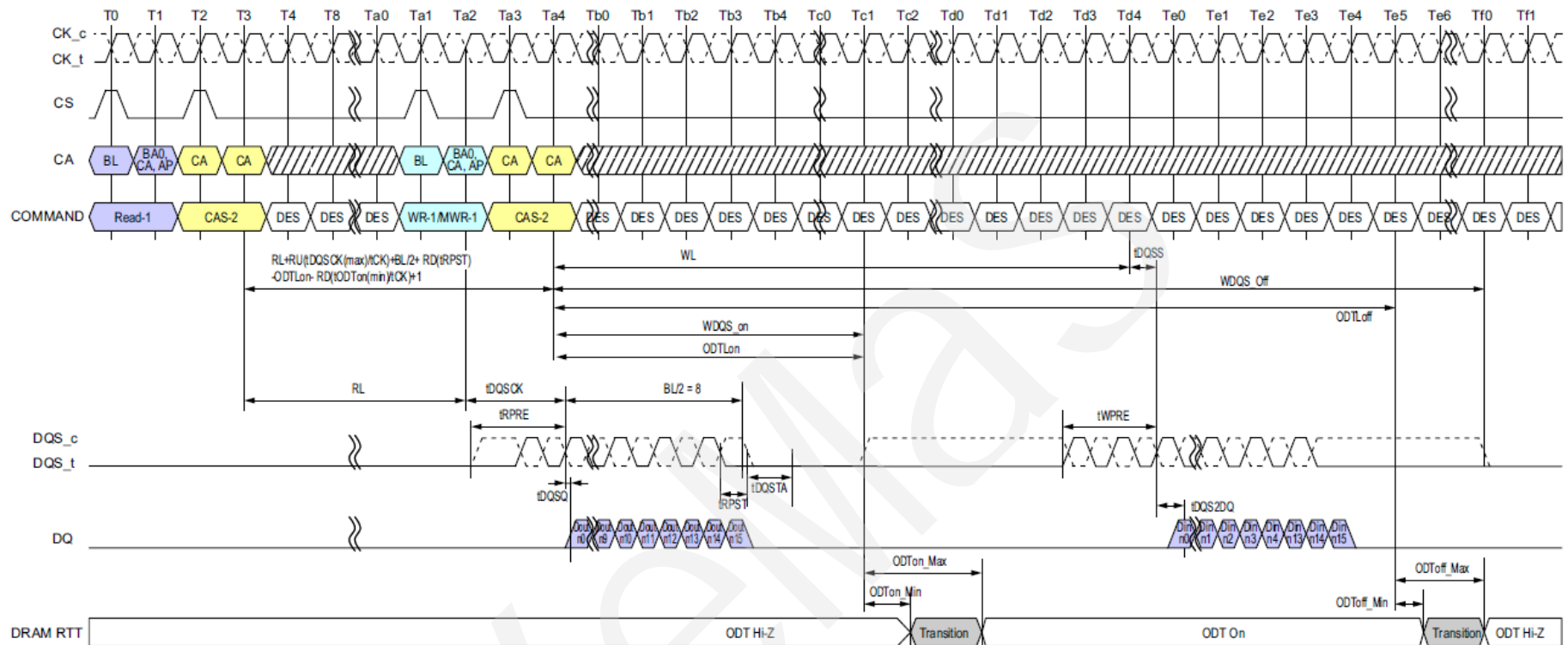
Figure 63 - Burst Read followed by Burst Write or Burst Mask Write (ODT Enable)
