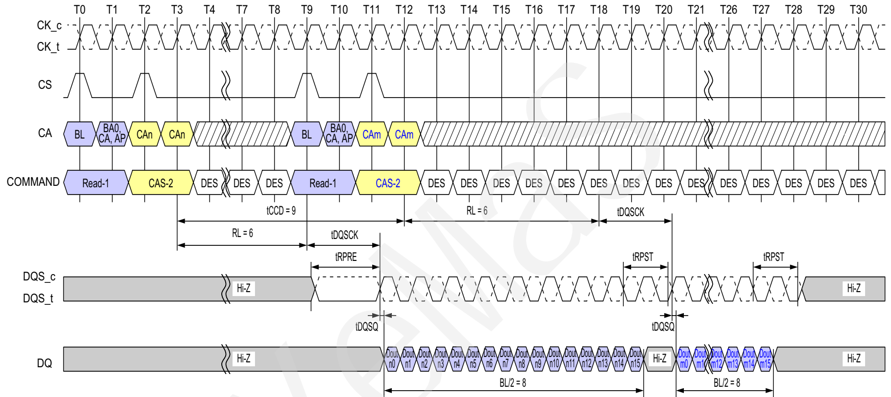
Figure 29 - Consecutive Reads Operation: t_{CCD} = \text{Min} + 1 , Preamble = Static, 1.5nCK Postamble
