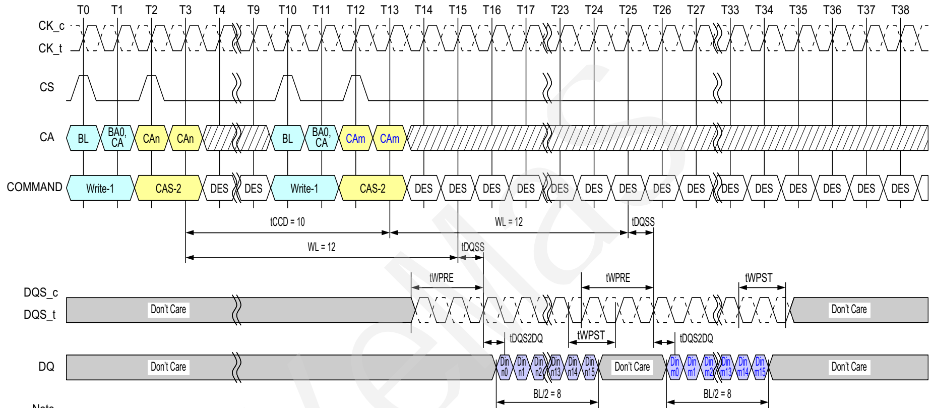
Figure 45 - Consecutive Writes Operation: t_{CCD} = \text{Min} + 2, 1.5n\text{CK} Postamble
