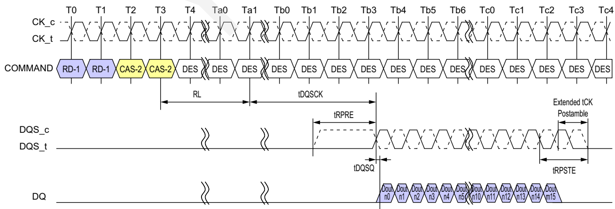
Figure 7 - DQS Read Preamble and Postamble: Static Preamble and 1.5nCK Postamble
