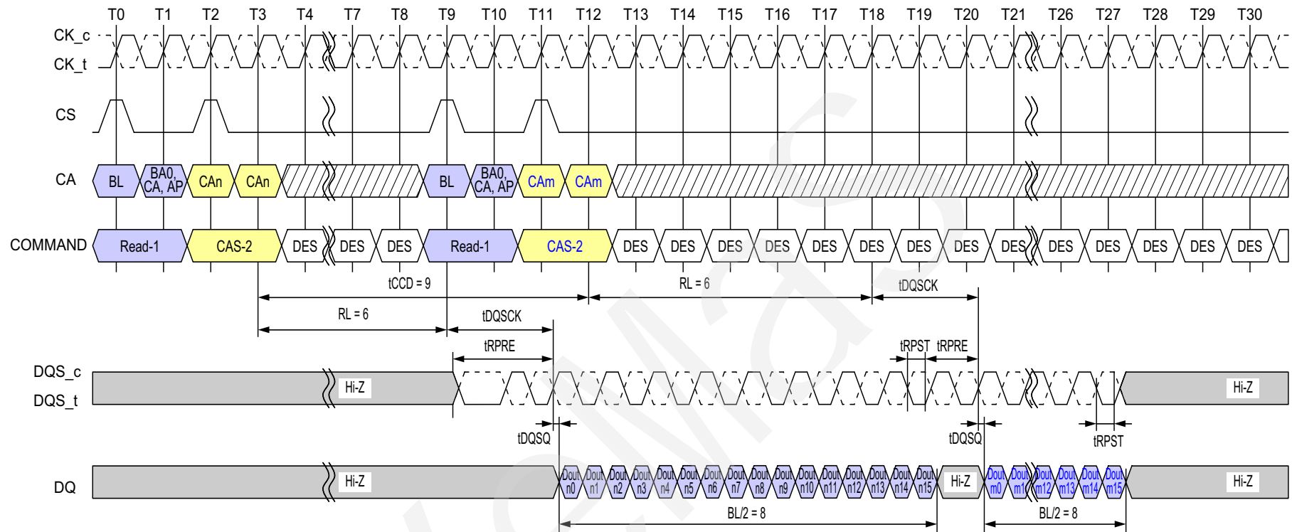
Figure 28 - Consecutive Reads Operation: tCCD=Min+1, Preamble=Toggle, 0.5nCK Postamble
