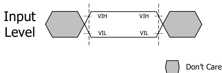
Figure 147 - Input AC timing definition for Reset_n and ODT_CA
