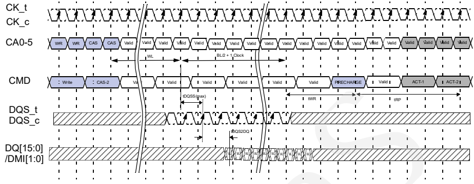
Figure 55 - Burst Write followed by Precharge (BL16, 2tCK Preamble)
