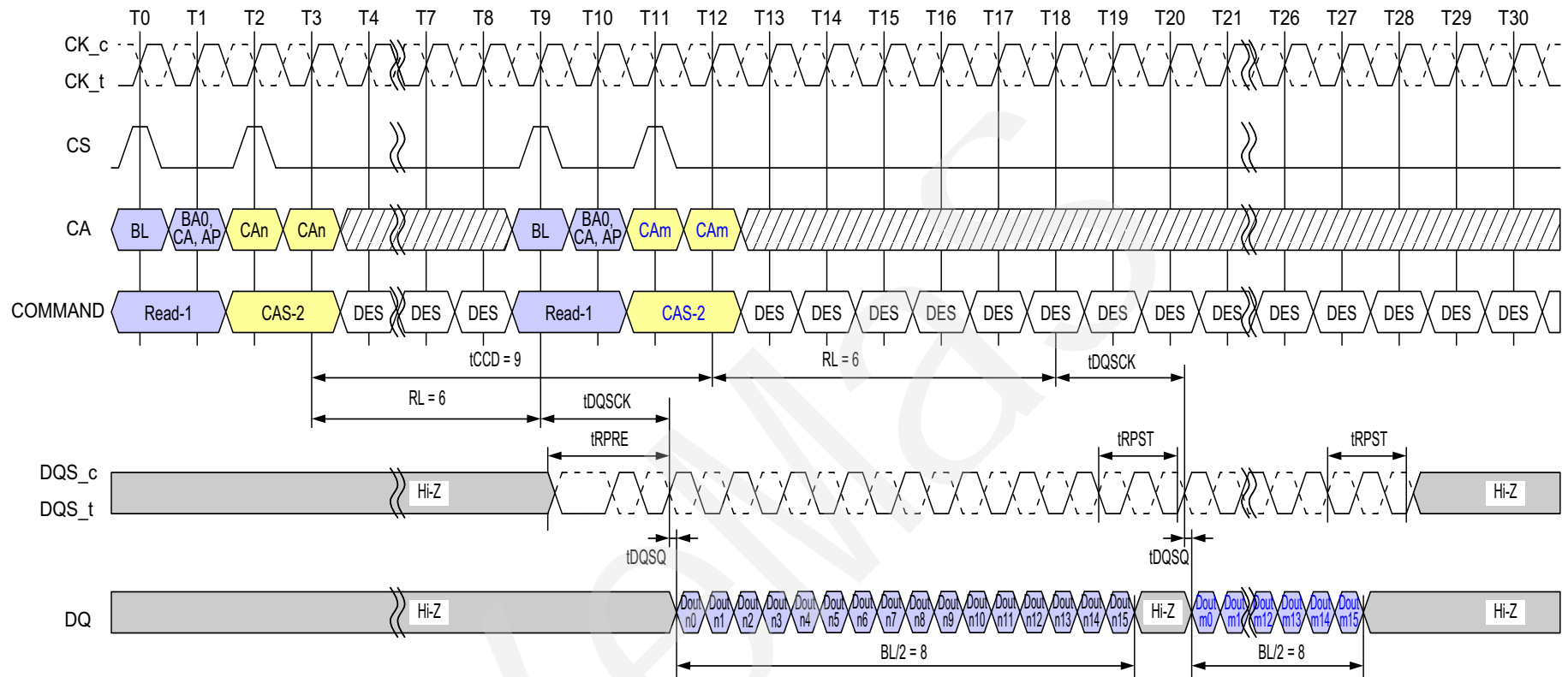
Figure 27 - Consecutive Reads Operation: t_{CCD} = \text{Min}+1 , Preamble=Toggle, 1.5n\text{CK} Postamble
