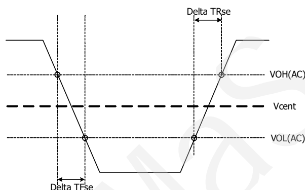
Figure 159 - Single Ended Output Slew Rate Definition
