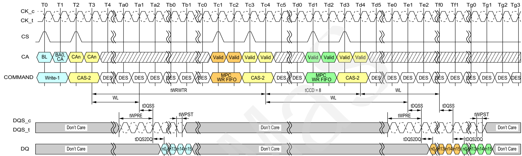
Figure 112 - MPC [Write DQ FIFO] Operation Timing
