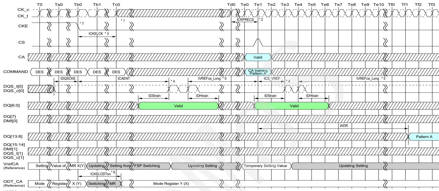
Figure 99 - Consecutive VrefCA Value Update
