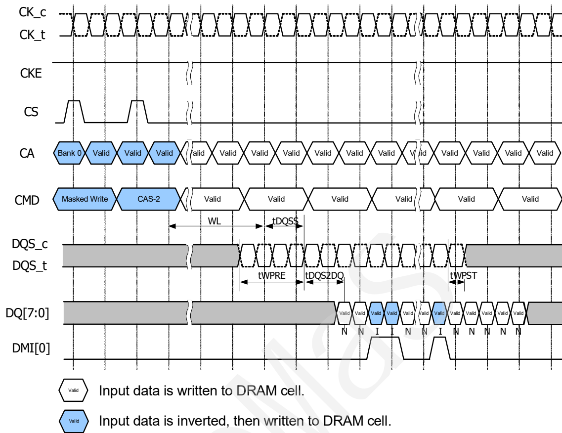
Figure 52 - Write Command w/ Write DBI Enabled; DM Disabled
