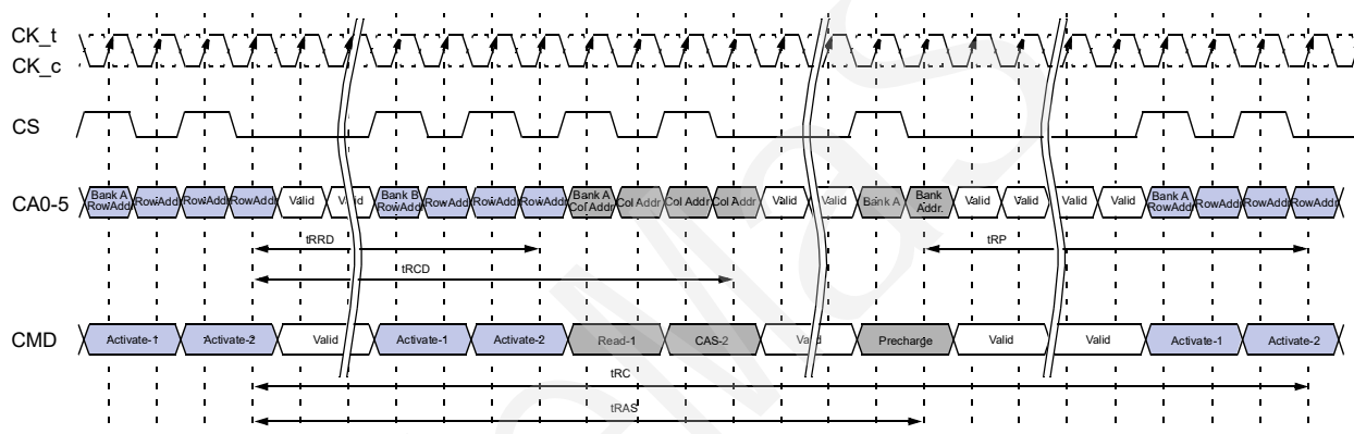
Figure 4 - Activate Command Timing Example
