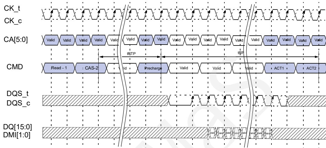
Figure 53 - Burst Read followed by Precharge (BL16, Toggling Preamble)
