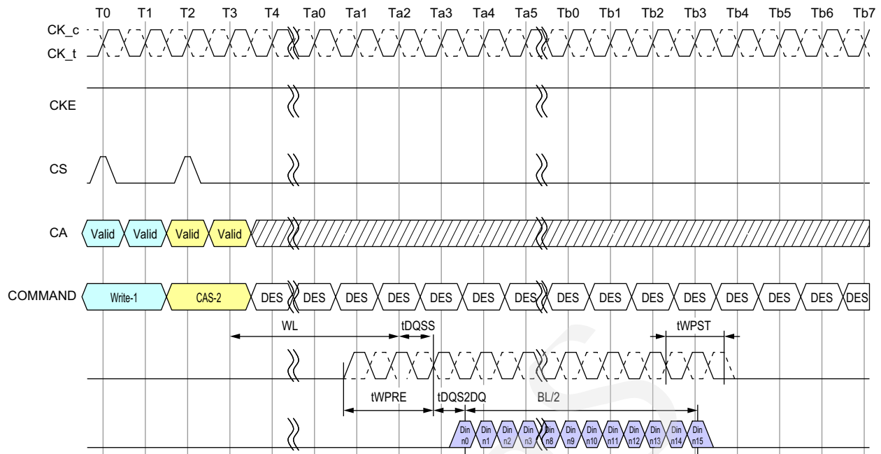
Figure 20 - DQS Write Preamble and Postamble: 1.5nCK Postamble
