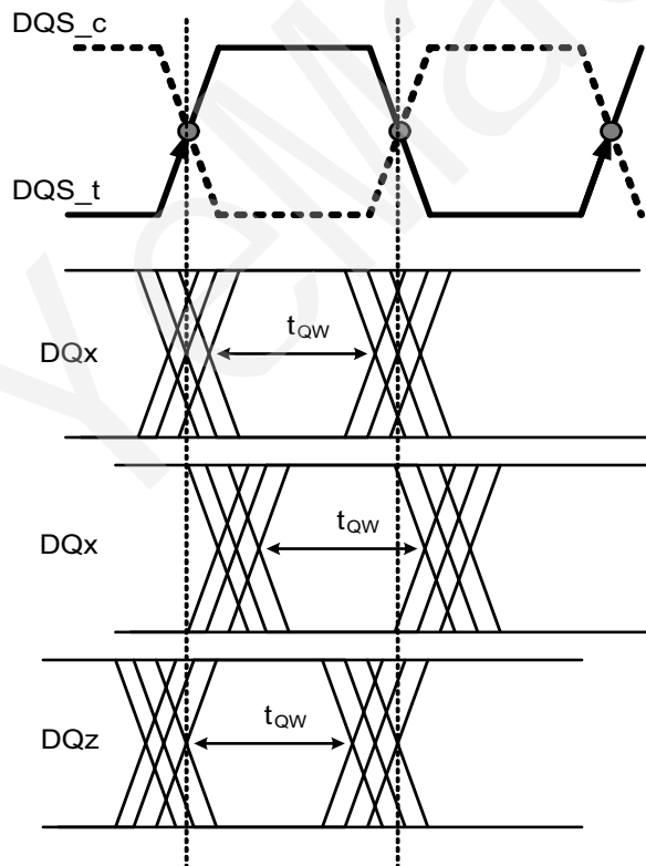
Figure 174 - Read data timing t_{QW} valid window defined per DQ signal
