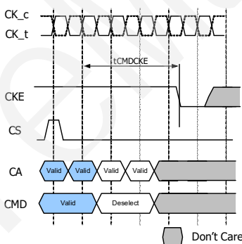
Figure 167 - tCMDCKE Timing
