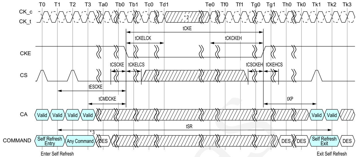
Figure 73 - Self Refresh Entry/Exit Timing with Power Down Entry/Exit
