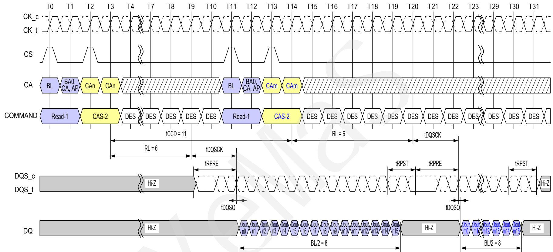
Figure 35 - Consecutive Reads Operation: t_{CCD} = \text{Min} + 3 , Preamble = Toggle, 1.5n\text{CK} Postamble
