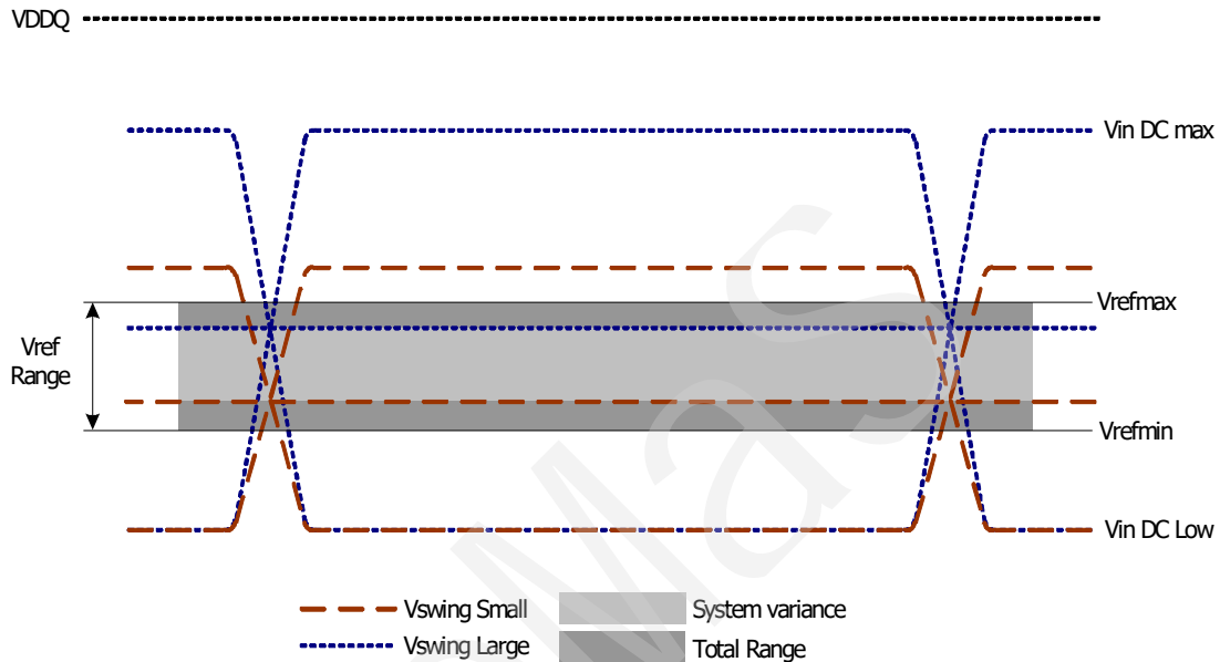
Figure 91 - Vref operating range (Vref.min, Vref.max)
