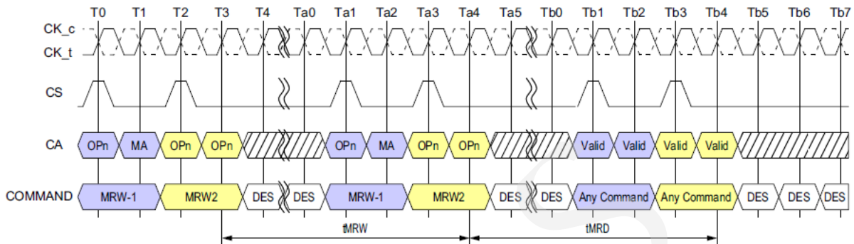
Figure 81 - Mode Register Write Timing
