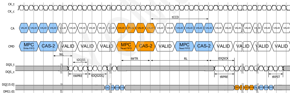
Figure 122 - MPC [RD FIFO] Read Operation (Shown with tWPST=0.5nCK, tRPRE=toggling, tRPST=1.5nCK)
