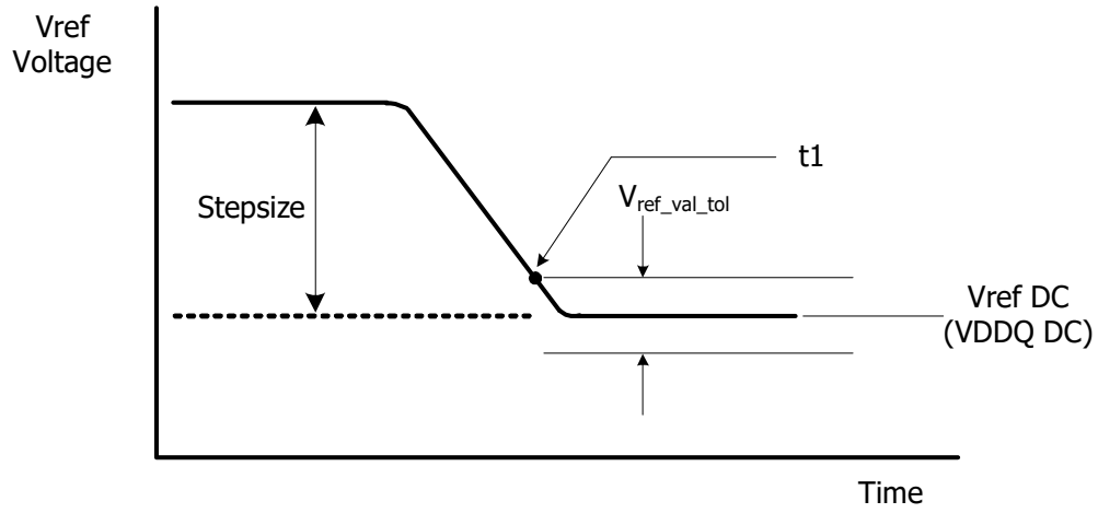
Figure 88 - Vref step single step size decrement case
