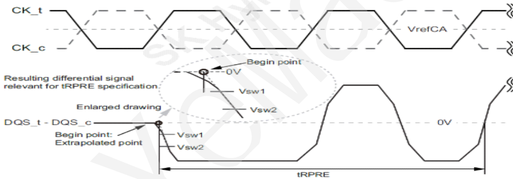
Figure 17 - Method for calculating tRPRE transitions and endpoints 2
