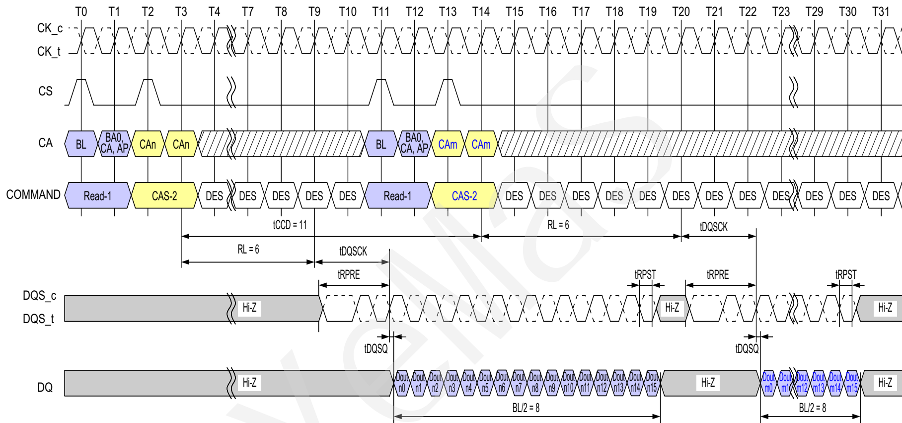
Figure 36 - Consecutive Reads Operation: t_{CCD} = \text{Min} + 3 , Preamble = Toggle, 0.5n\text{CK} Postamble
