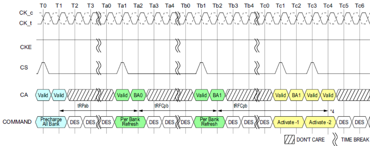
Figure 65 - Per-Bank REFRESH to a different bank Operation
