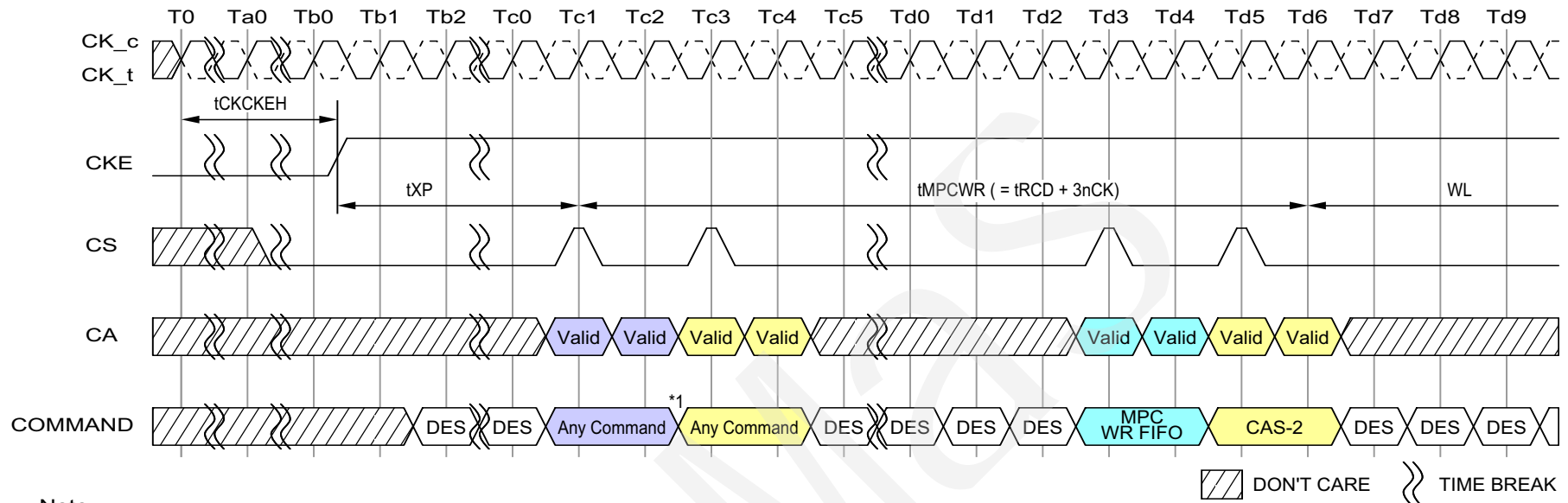
Figure 116 - Power Down Exit to MPC [Write FIFO] Timing
