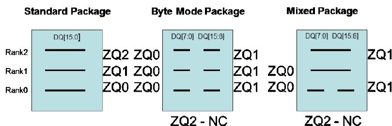
Figure 126 - ZQ Wiring Overview
