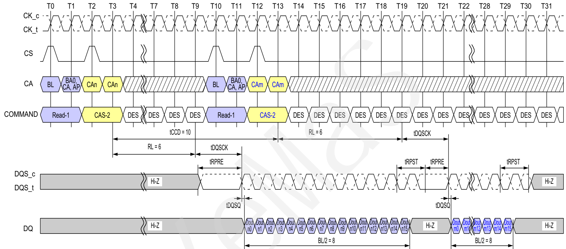
Figure 33 - Consecutive Reads Operation: t_{CCD} = \text{Min} + 2 , Preamble = Static, 1.5nCK Postamble
