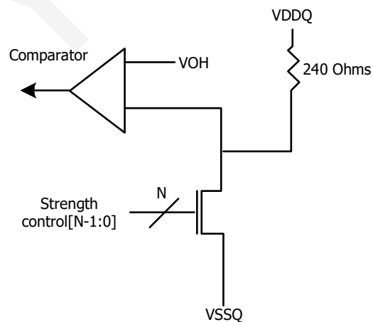
Figure 164 - Pull-down calibration
