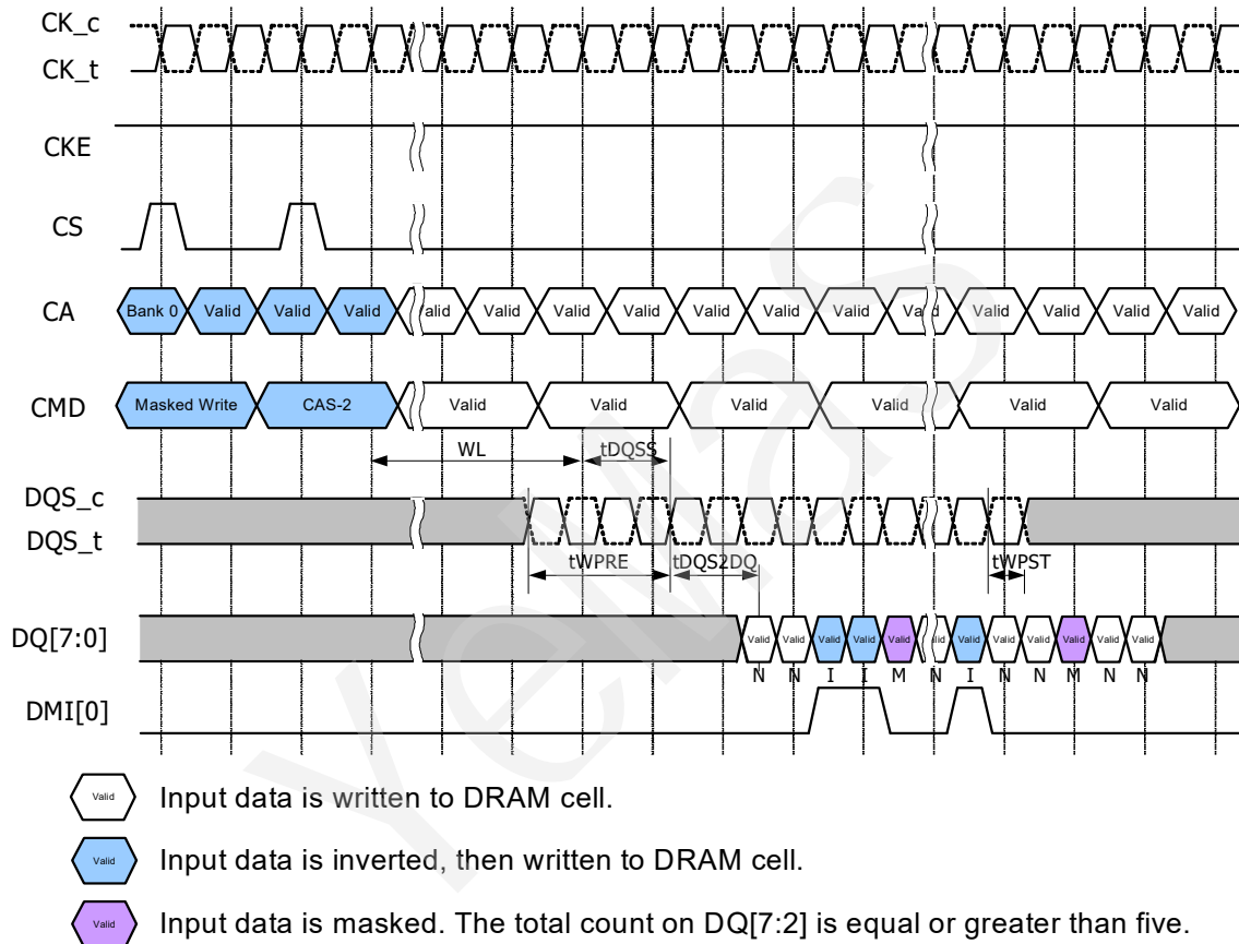
Figure 51 - Masked Write Operation w/ Write DBI Enabled; DM Enabled
