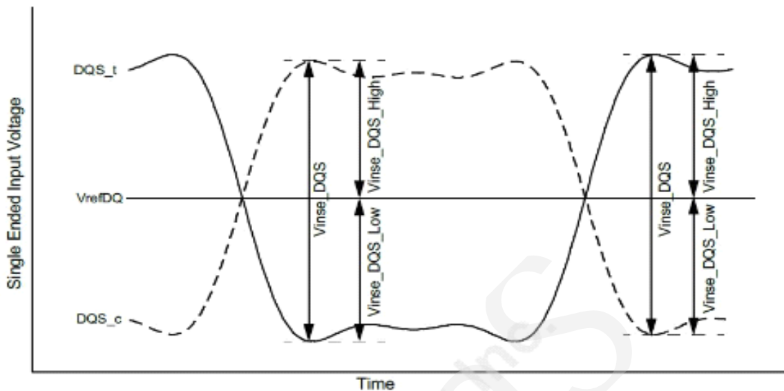
Figure 156 - DQS Single-Ended Input Voltage
