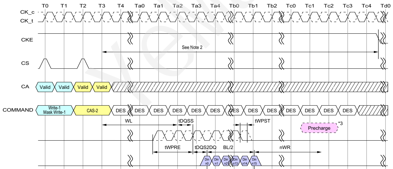
Figure 137 - Write and Masked Write with Auto Precharge to Power-Down Entry
