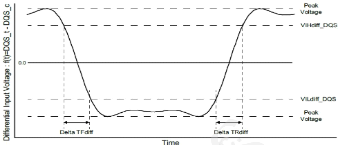
Figure 157 - Differential Input Slew Rate Definition for DQS t , DQS c
