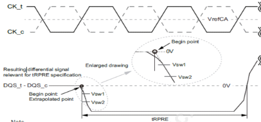
Figure 16 - Method for calculating tRPRE transitions and endpoints
