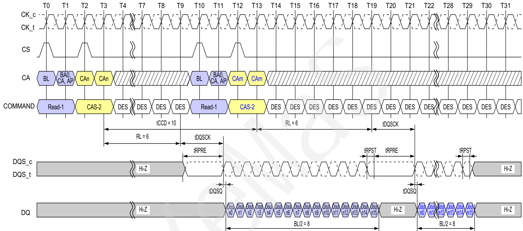
Figure 34 - Consecutive Reads Operation: t_{CCD} = \text{Min} + 2 , Preamble = Static, 0.5nCK Postamble
