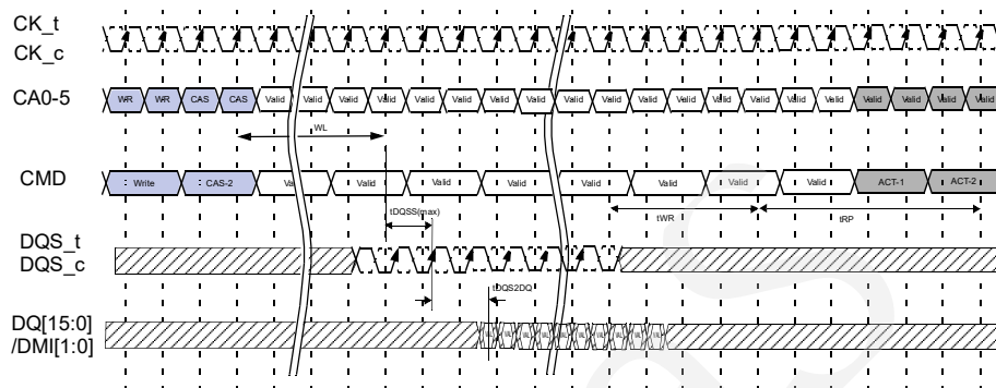
Figure 59 - Burst Write with Auto-Precharge (BL16, 2tCK preamble)
