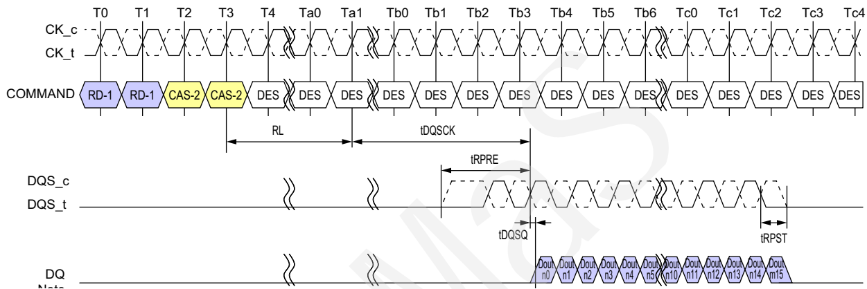
Figure 6 - DQS Read Preamble and Postamble: Toggling Preamble and 0.5nCK Postamble
