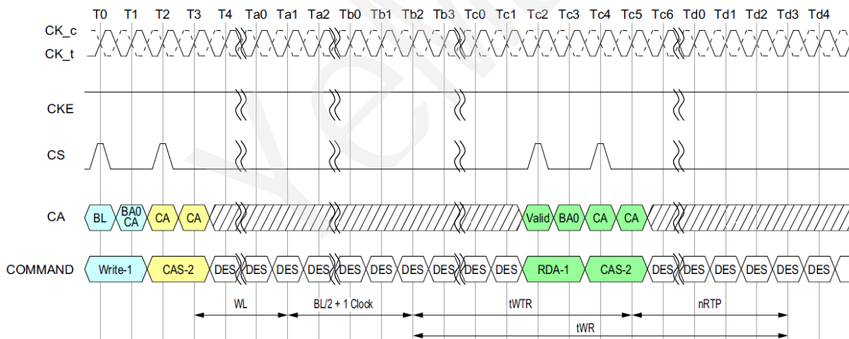
Figure 60 - Delay time from write to Read with Auto-Precharge
