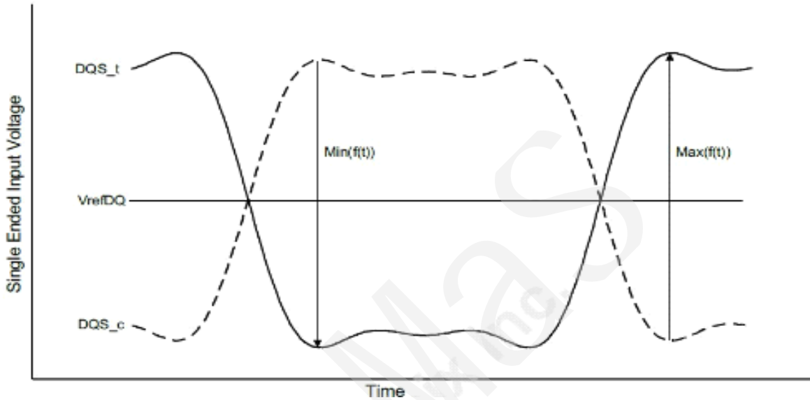
Figure 155 - Definition of differential DQS Peak Voltage
