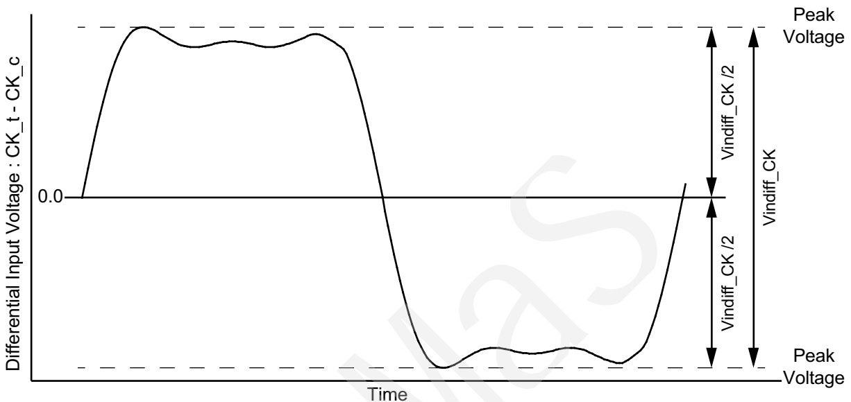
Figure 149 - CK Differential Input Voltage
