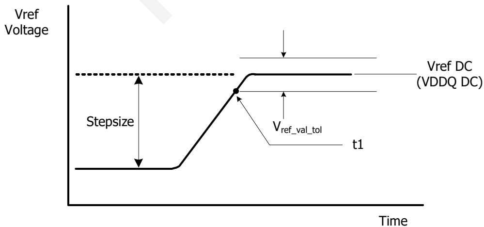
Figure 87 - Vref step single step size increment case
