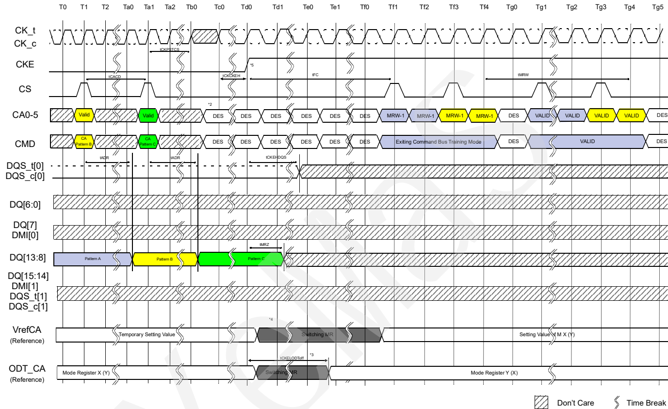
Figure 100 - Exiting Command Bus Training Mode with Valid Command
