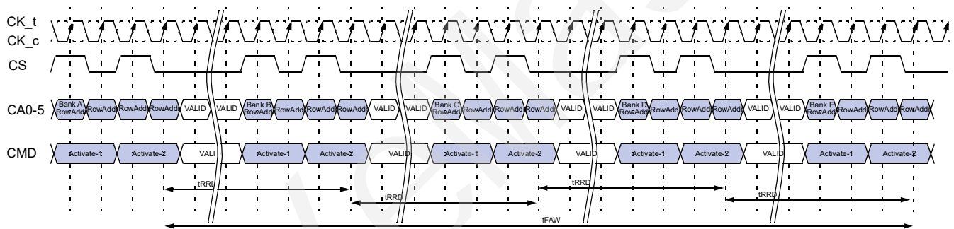
Figure 5 - tFAW Timing Example
