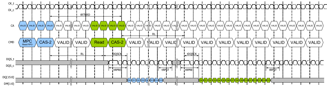
Figure 123 - MPC [RD FIFO] Operation (Shown with tRPRE=toggling, tRPST=1.5nCK)
