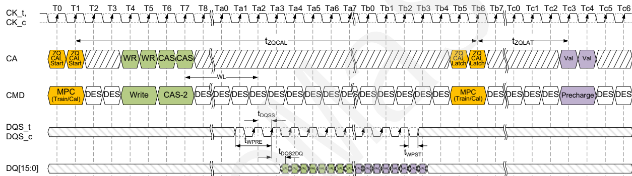
Figure 125 - ZQCal Timing
