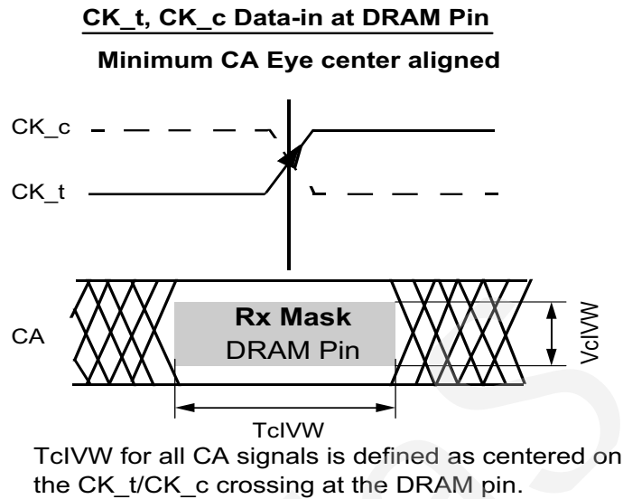
Figure 170 - CA Timing at the DRAM pins
