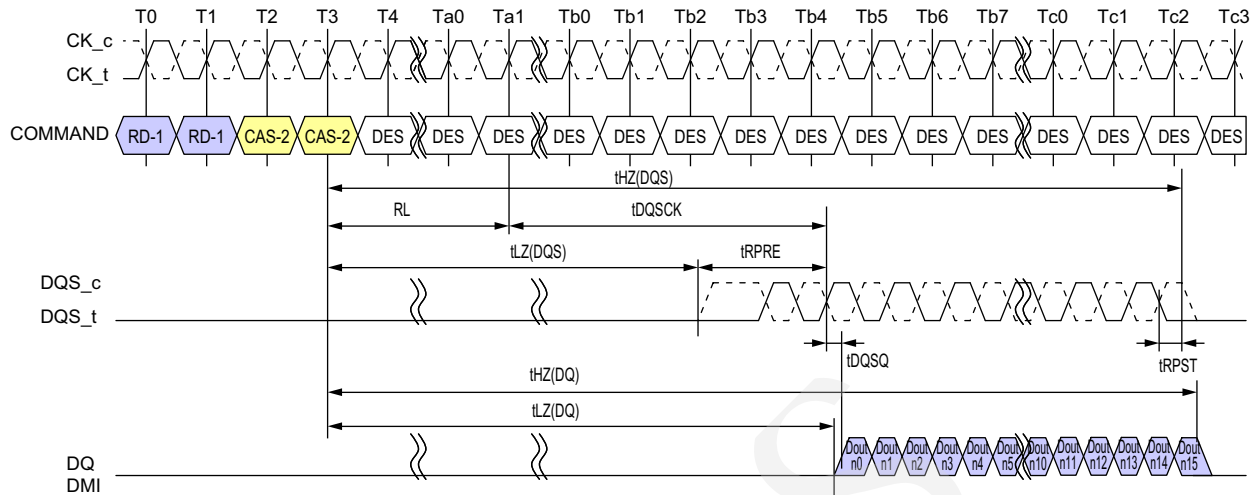
Figure 11 - Read Timing
