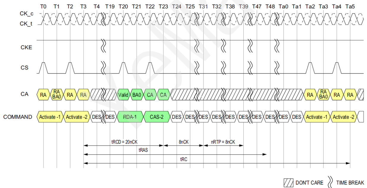
Figure 56 - Command Input Timing with RAS lock
