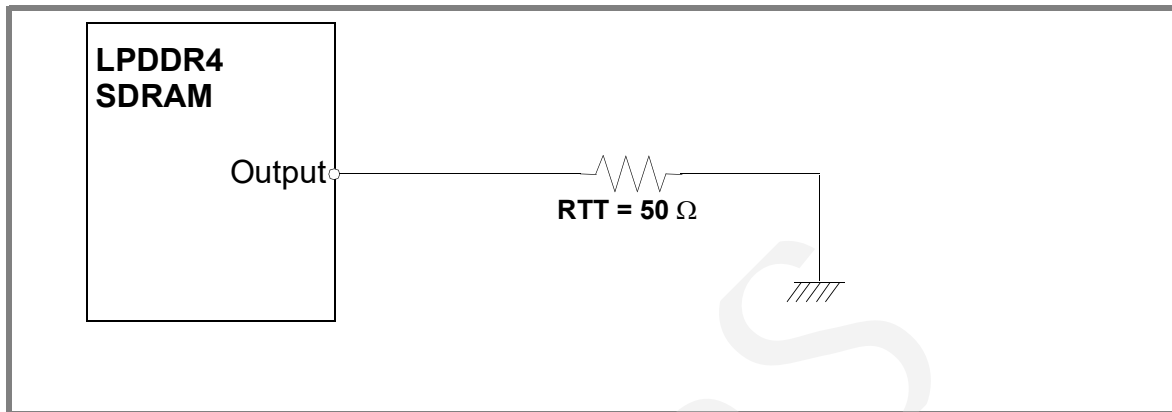
Figure 162 - Driver Output Reference Load for Timing and Slew Rate
