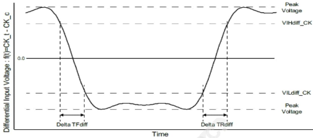
Figure 152 - Differential Input Slew Rate Definition for CK t , CK c
