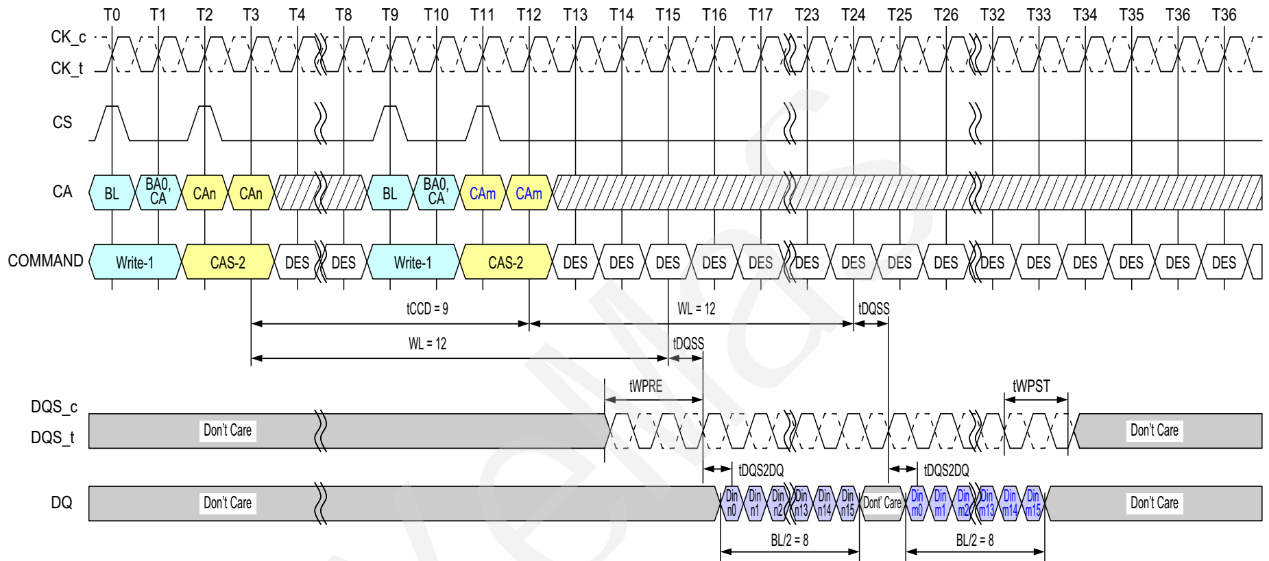
Figure 43 - Consecutive Writes Operation: t_{CCD} = \text{Min} + 1, 1.5nCK Postamble
