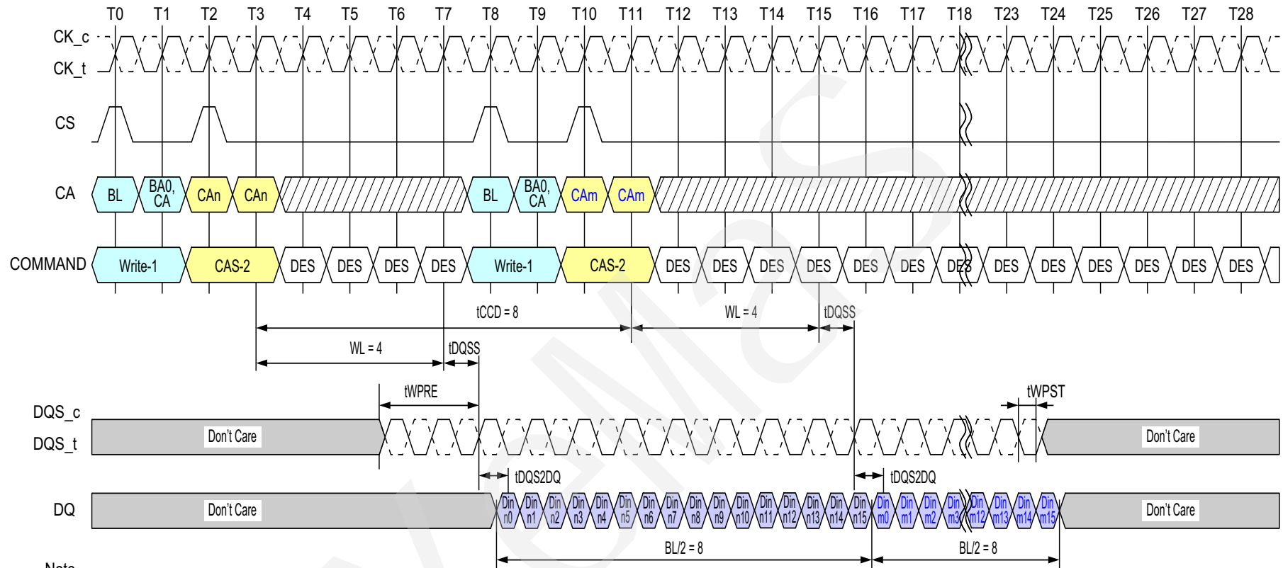
Figure 39 - Seamless Writes Operation: t_{CCD} = \text{Min}, 0.5n\text{CK} Postamble
