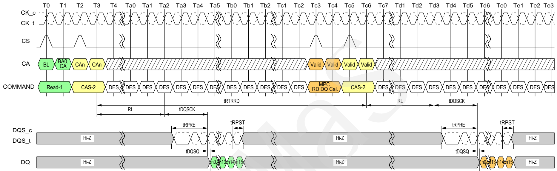
Figure 109 - DQ Read Training Timing: Read to Read DQ Calibration
