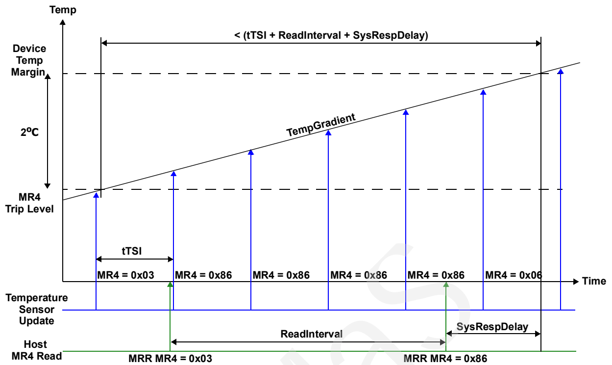
Figure 124 - Temp sensor Timing
