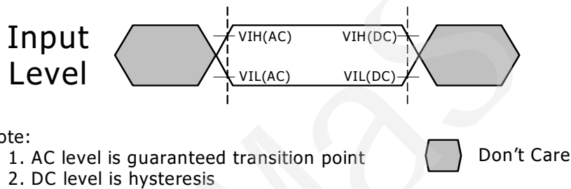
Figure 146 - Input AC timing definition for CKE
