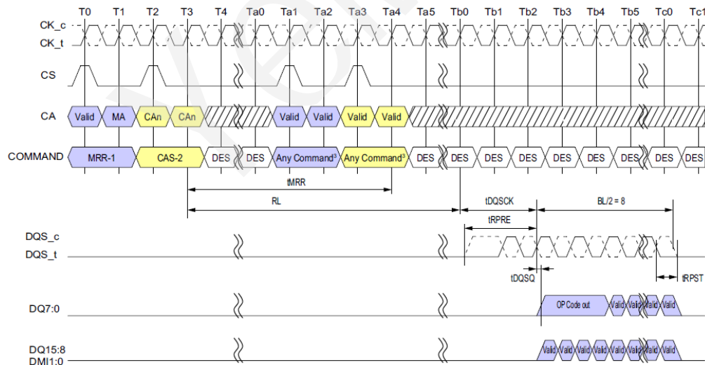
Figure 77 - Mode Register Read Operation
